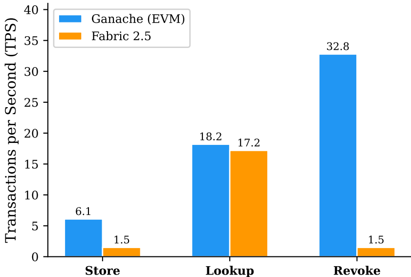
Throughput by Operation
