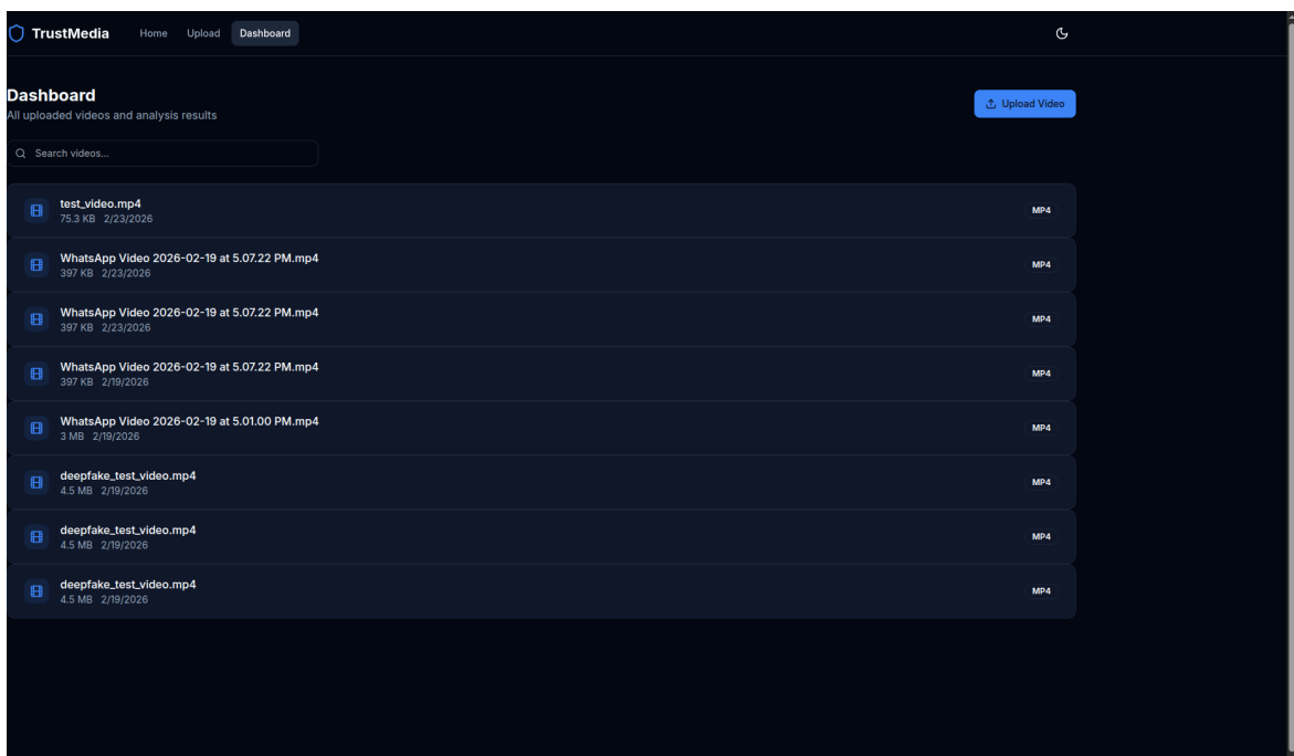
Figure 6.4: Videos Dashboard
