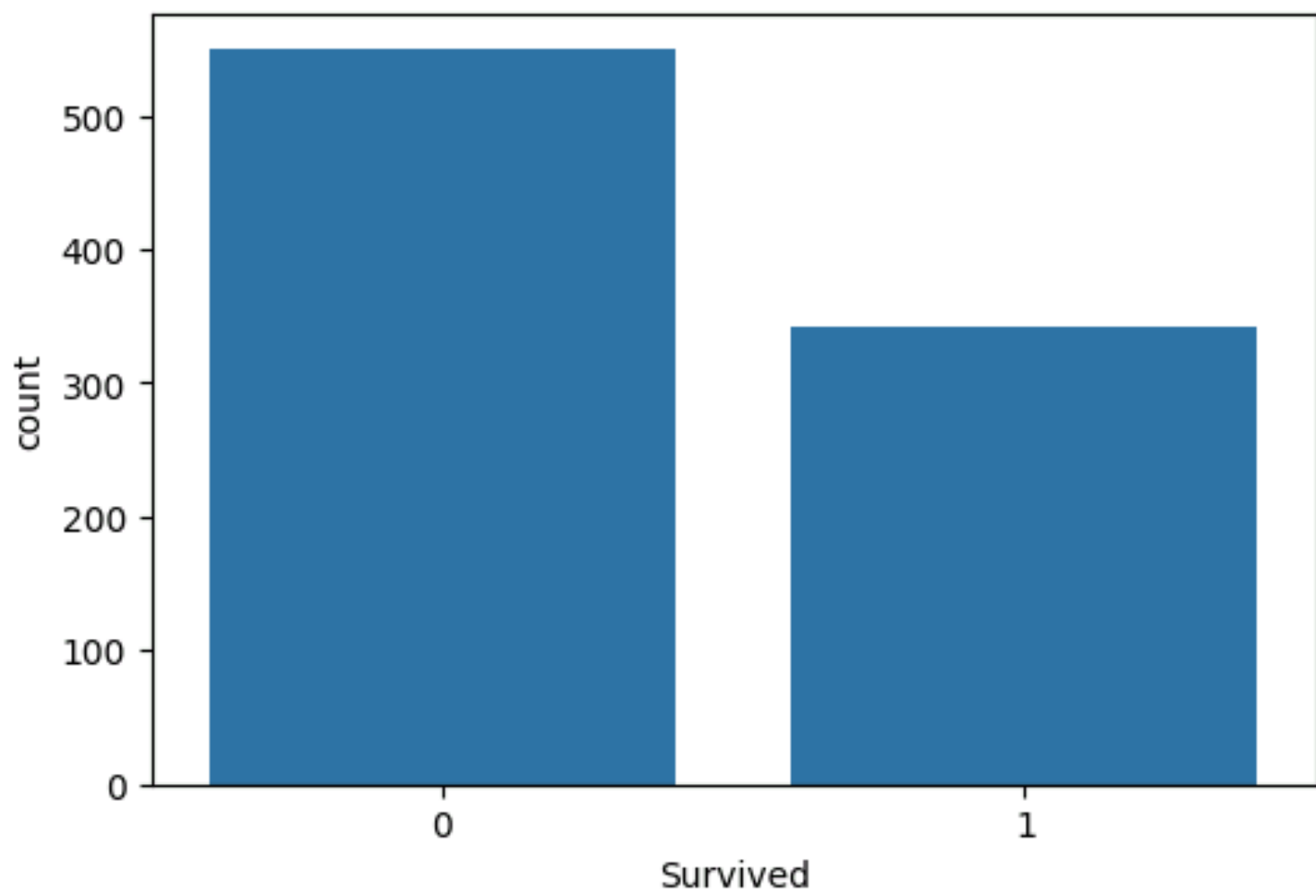
Survival Count
