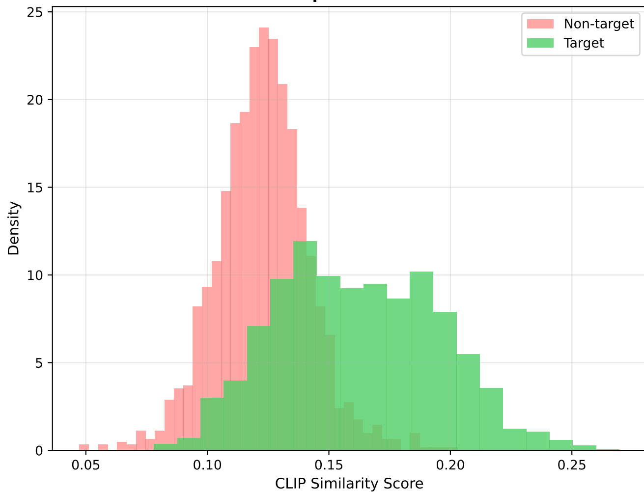
Adaptive Fusion
