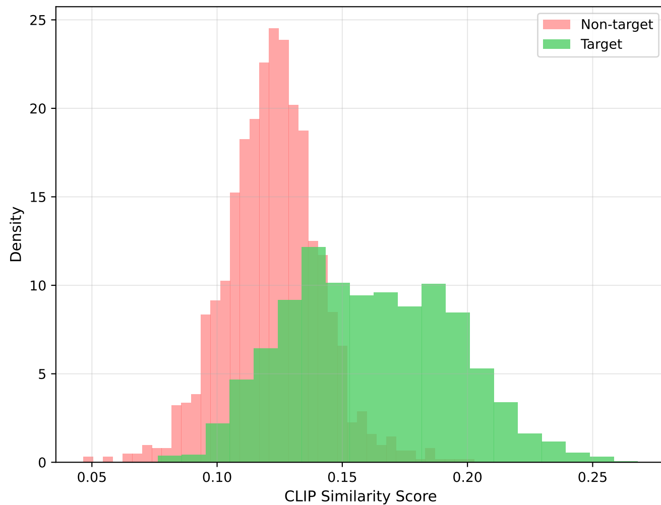
Mean Fusion
