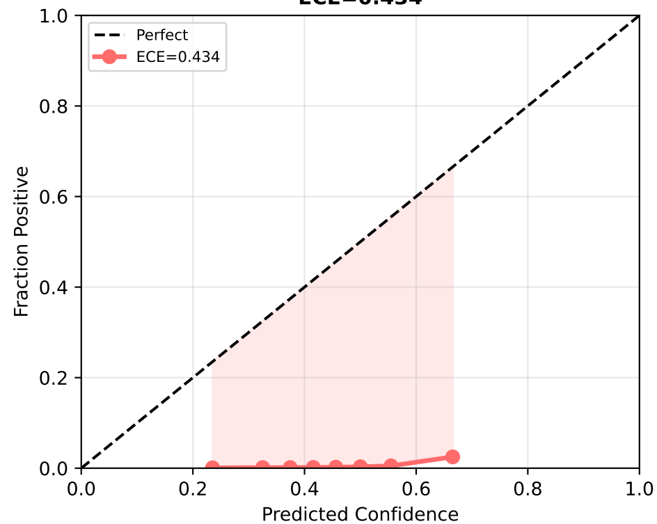
Baseline (Single) ECE=0.434
