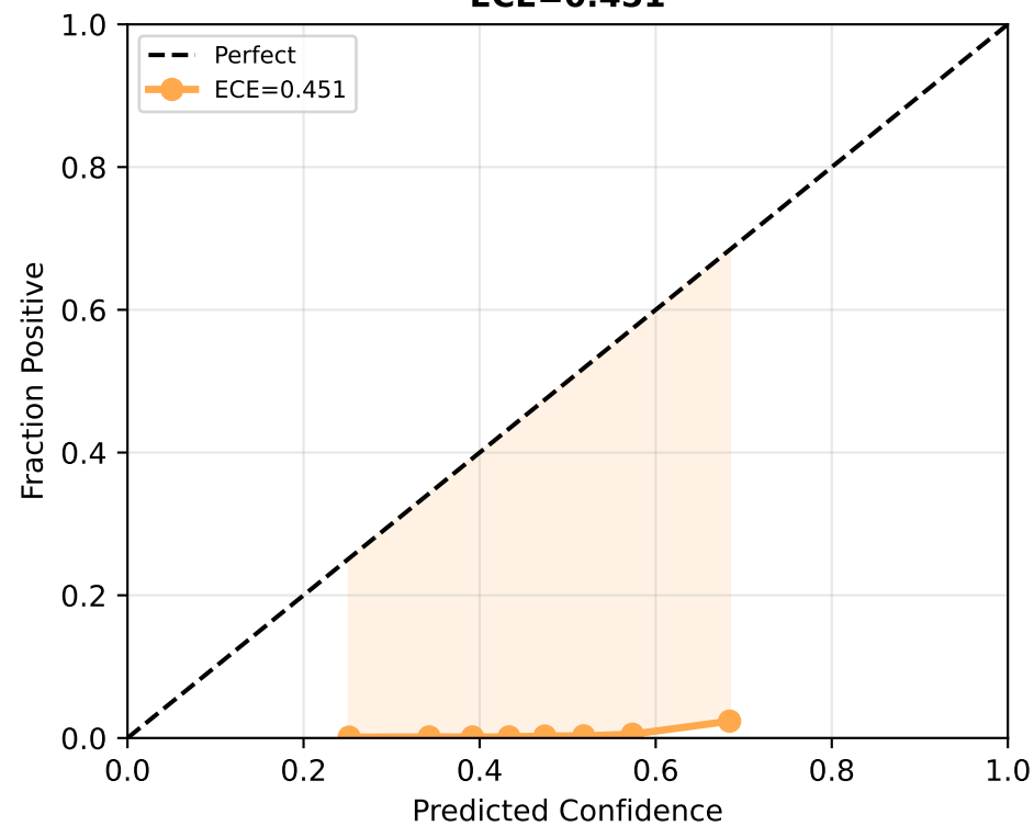
Mean Fusion ECE=0.451
