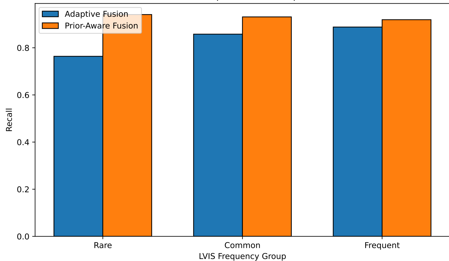
RQ5: Prior-Aware Fusion Improves LVIS Adaptive-Threshold Recall
