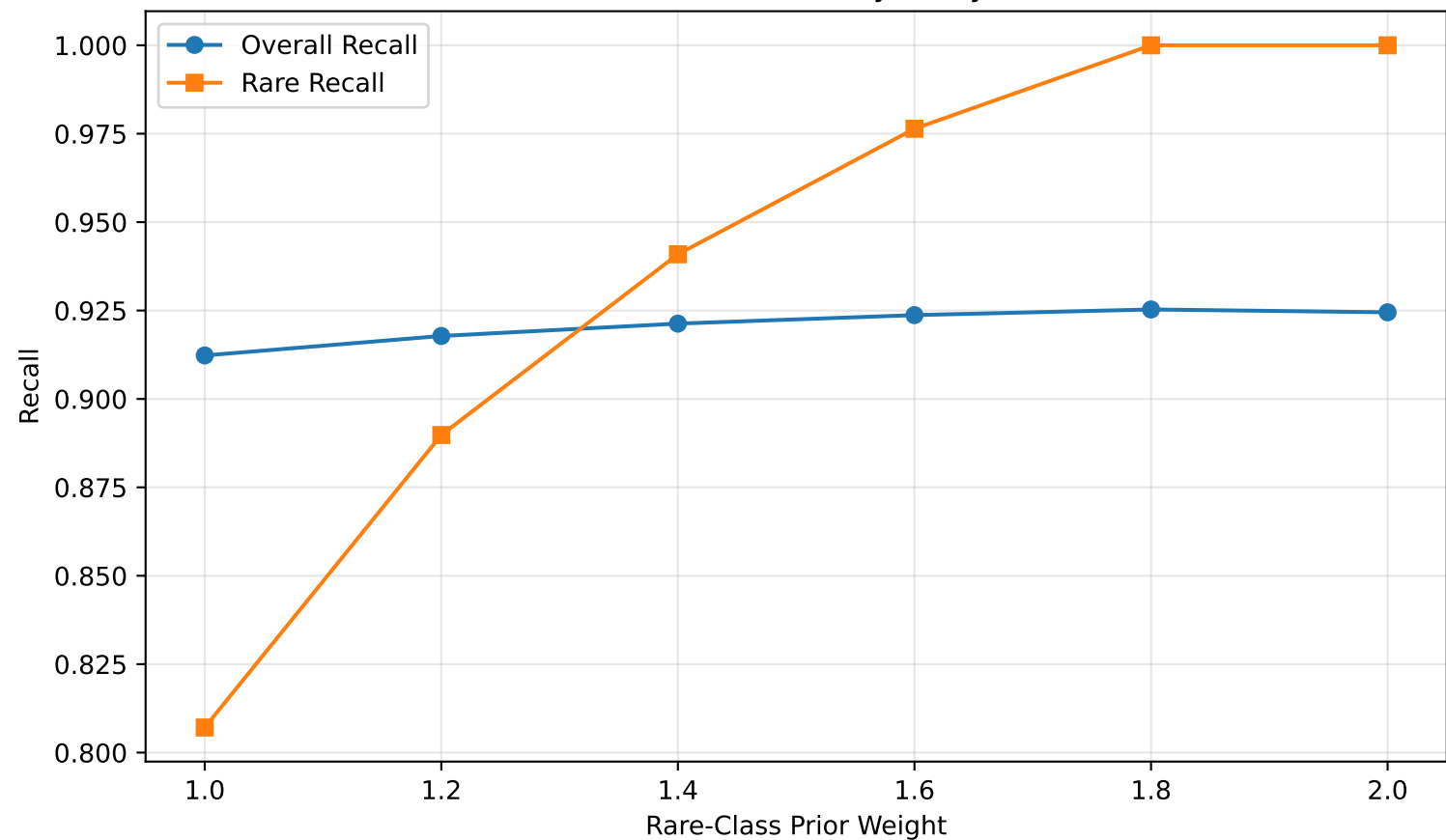
RQ5: Prior Sensitivity Analysis
