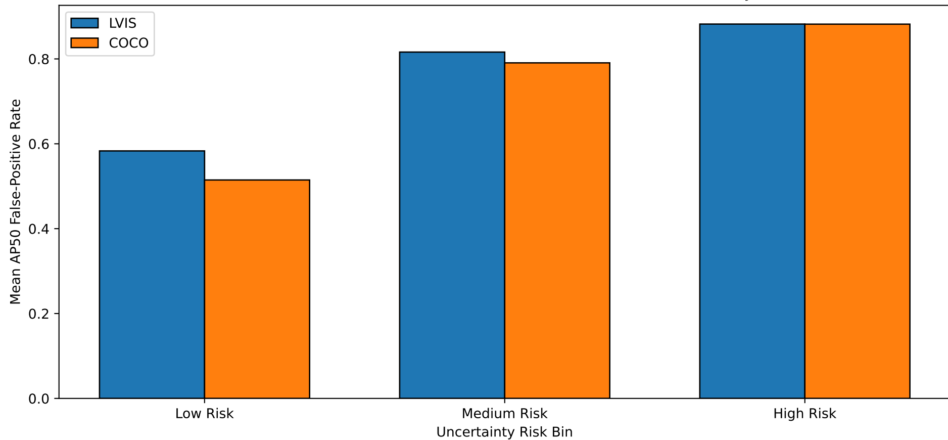
RQ3: False-Positive Rate Increases with Semantic Uncertainty
