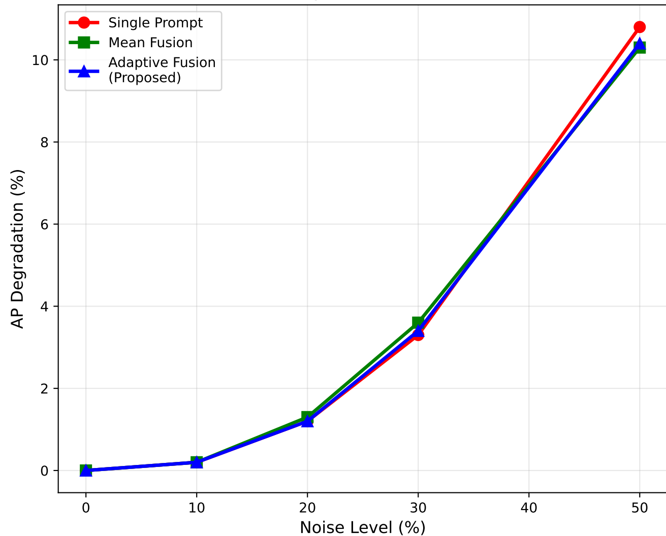
AP Degradation vs Noise
