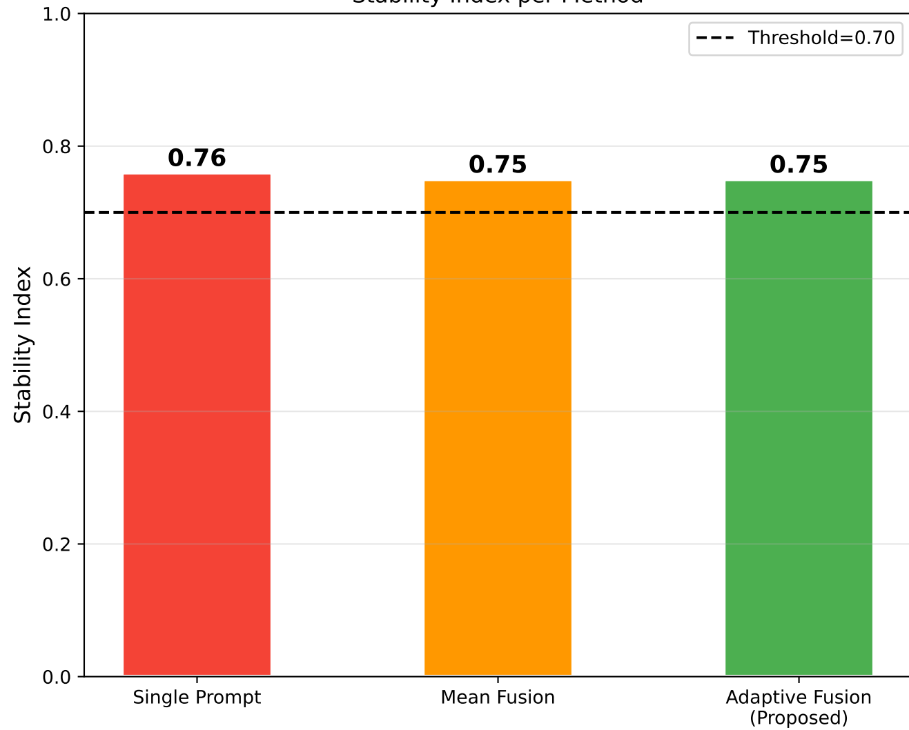
Stability Index per Method
