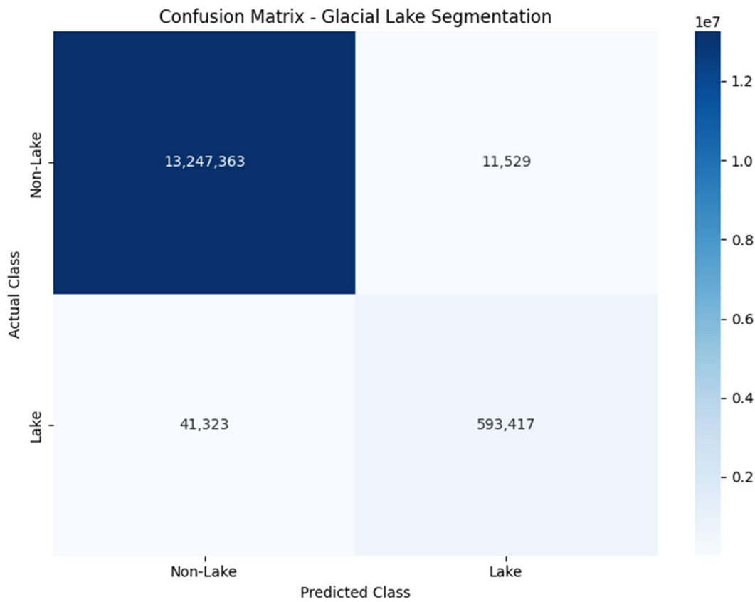
Fig.2:Confusion Matrix
