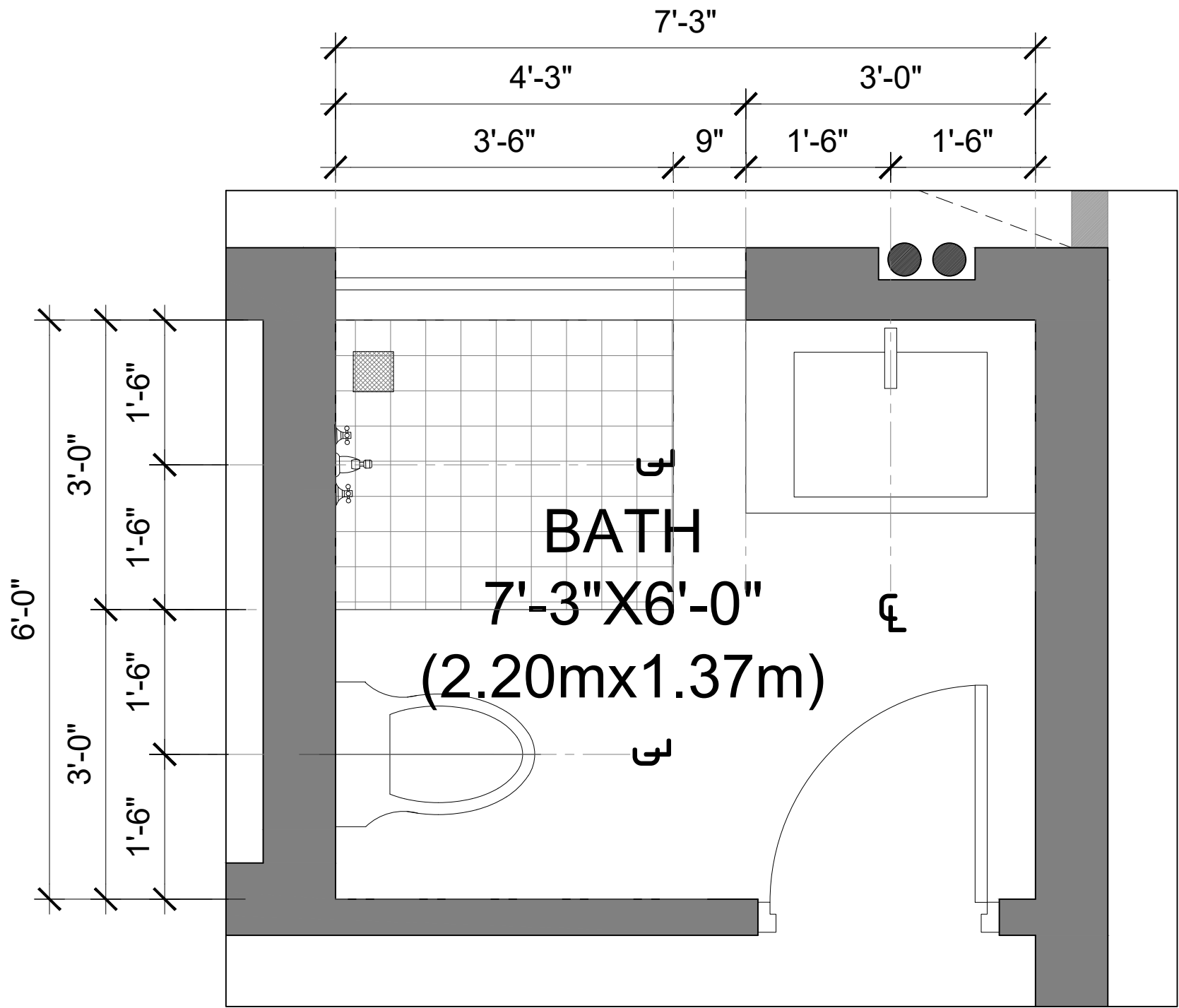
1 MUMTY FLOOR BATH
