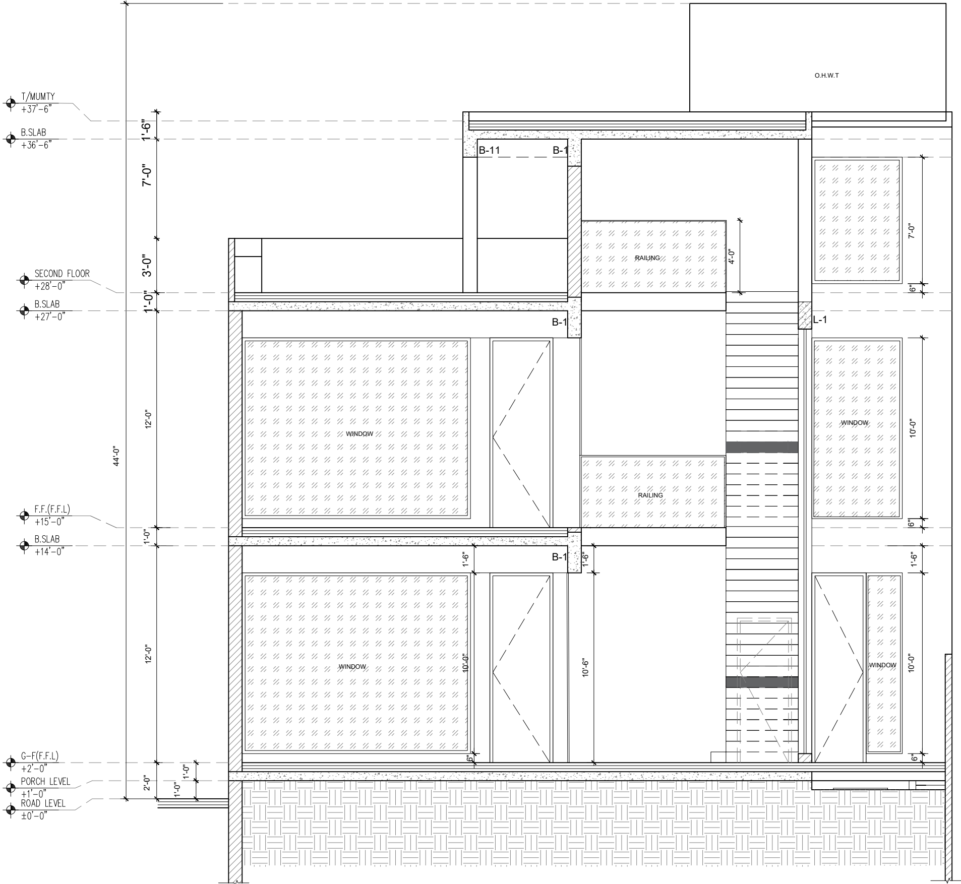
BB SECTION
