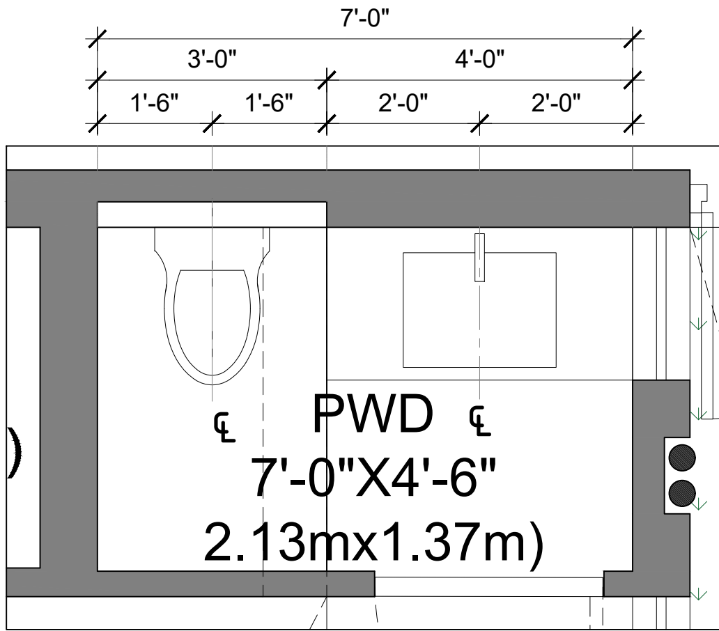
2 GROUND FLOOR PWD BATH
