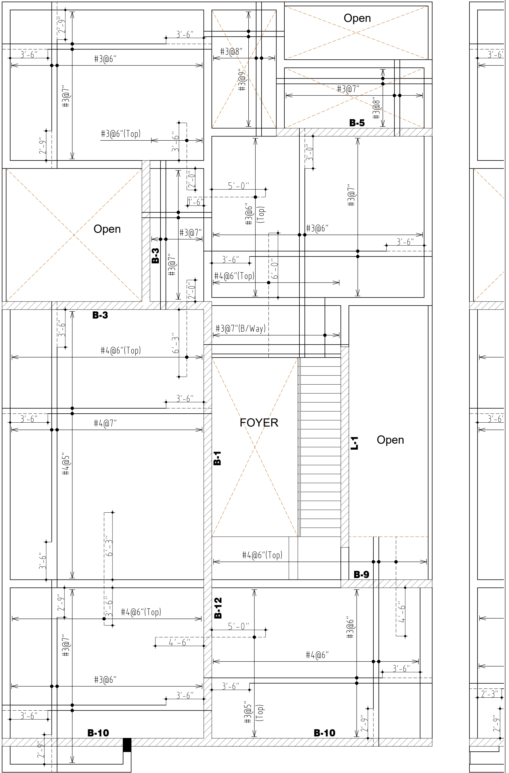
Renif: Plan of First Floor Slab. 6" Th: Slab.
