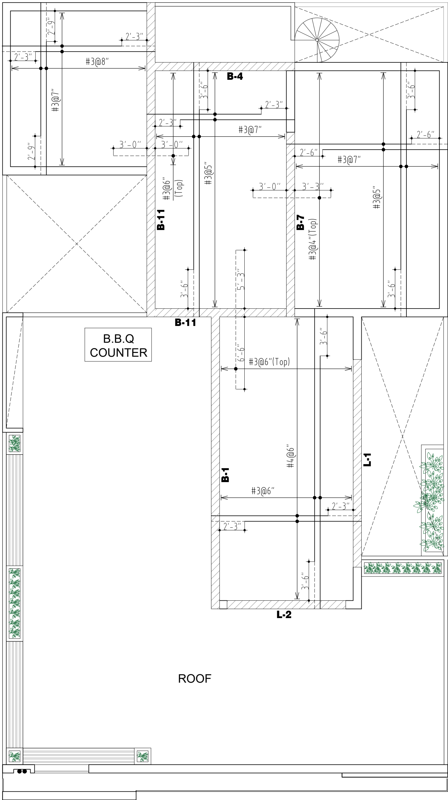
Renif: Plan of Mumty Slab. 6" Th: Slab.
