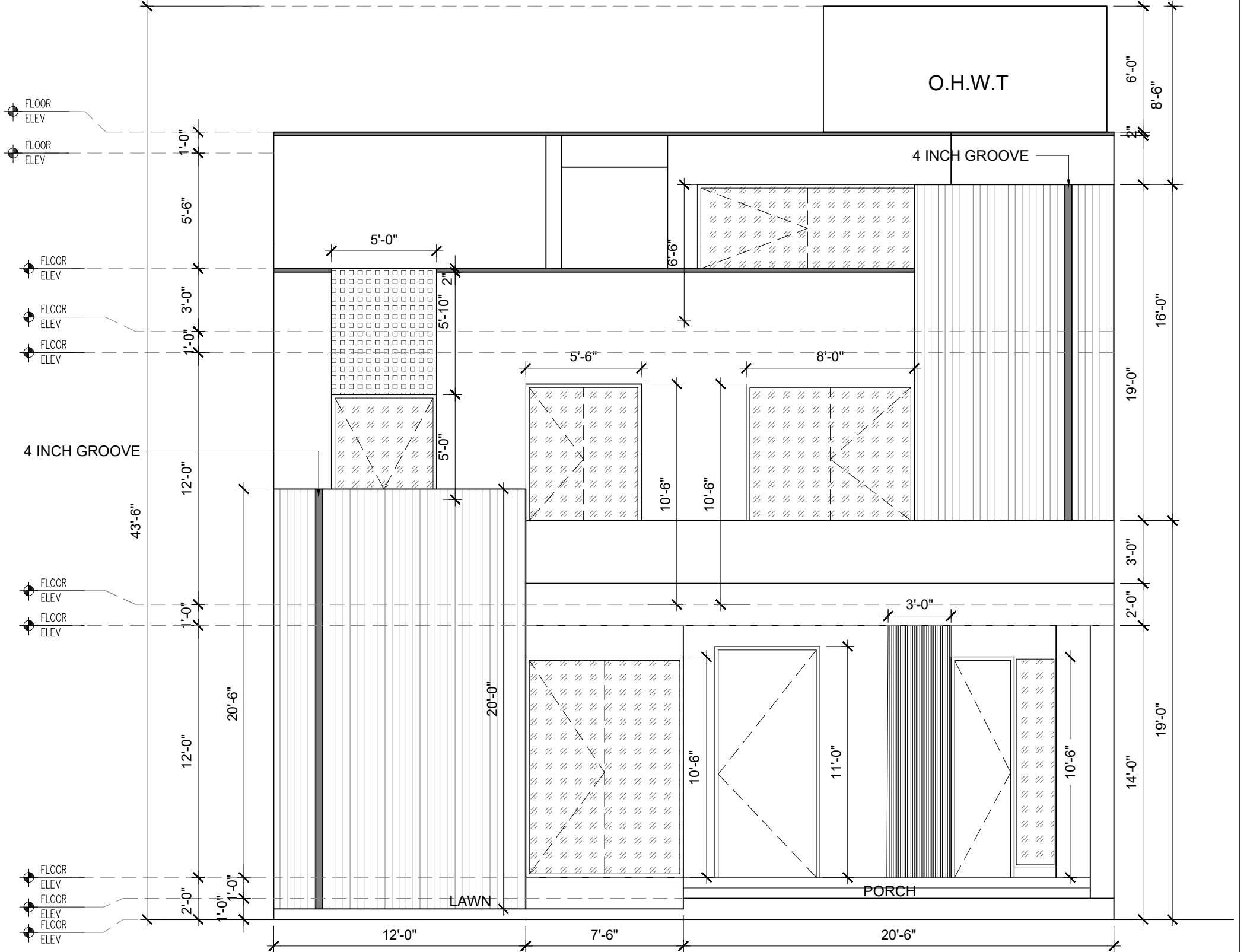
1 FRONT ELEVATION
