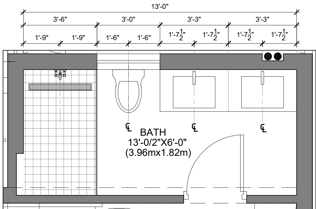
2 FIRST FLOOR BATH 2
