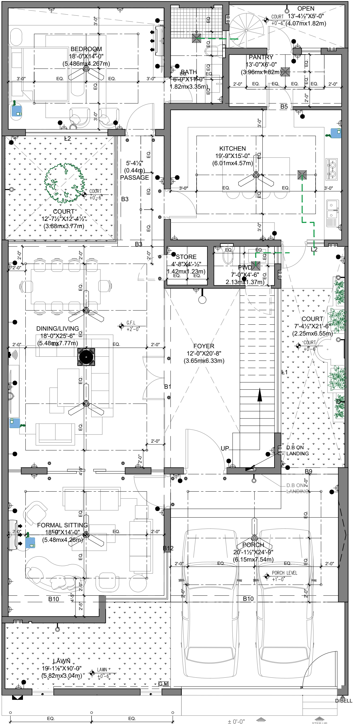
1 GROUND FLOOR ELECTRICAL LAYOUT PLAN AREA : 2220 SFT
