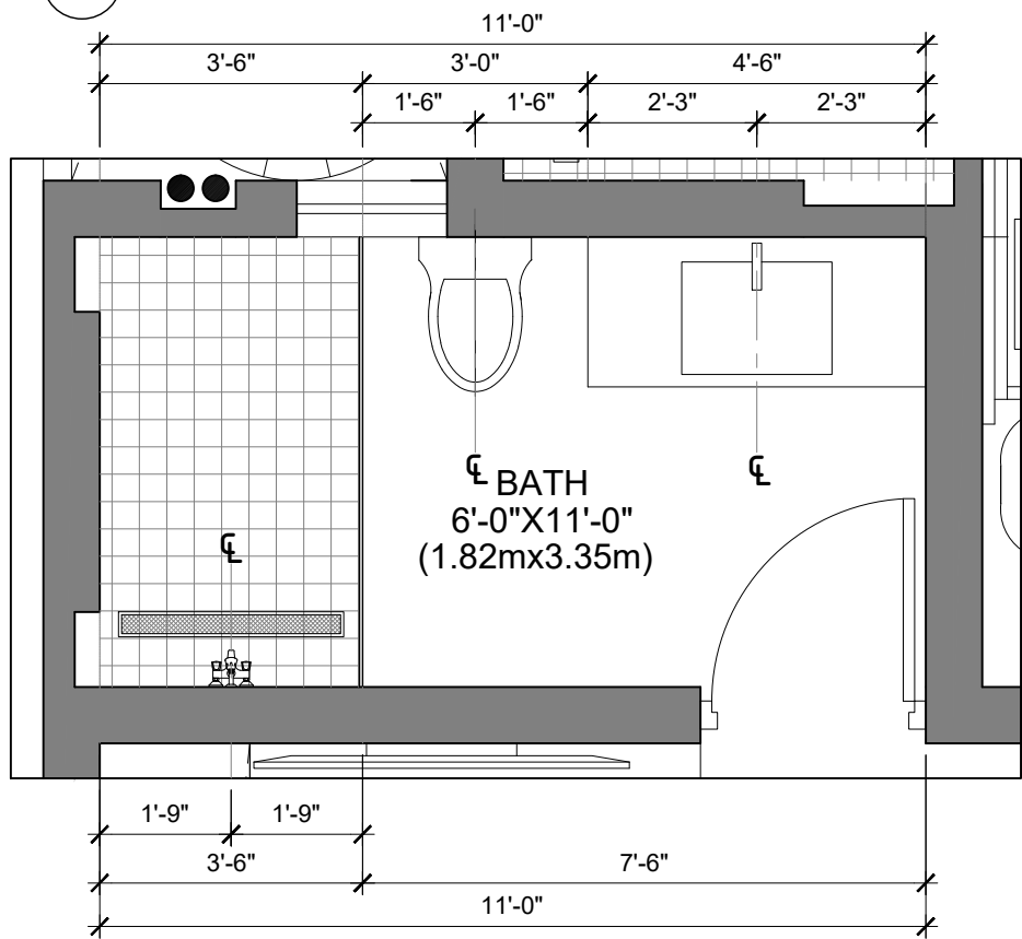
3 FIRST FLOOR BATH 3
