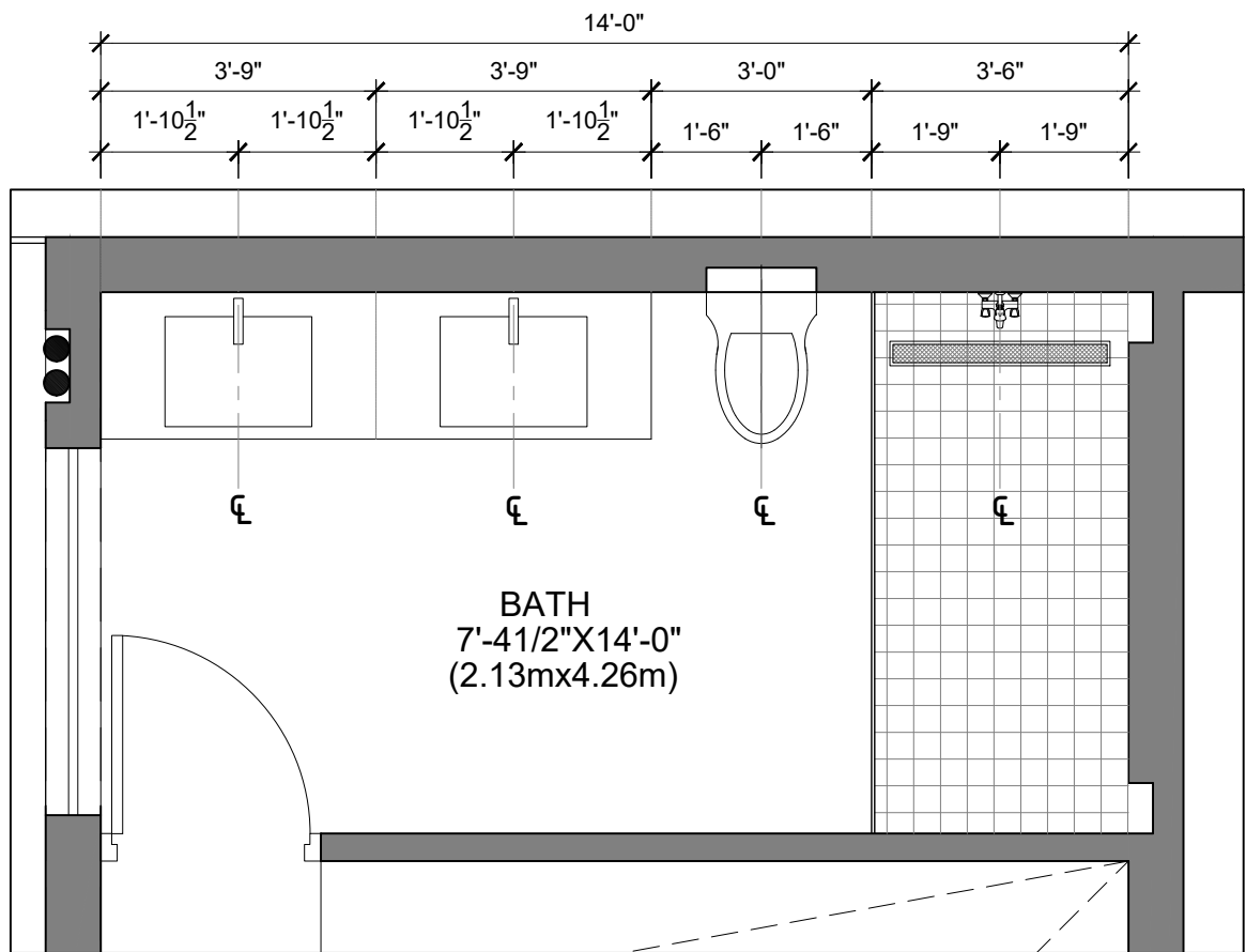
1 FIRST FLOOR BATH 1
