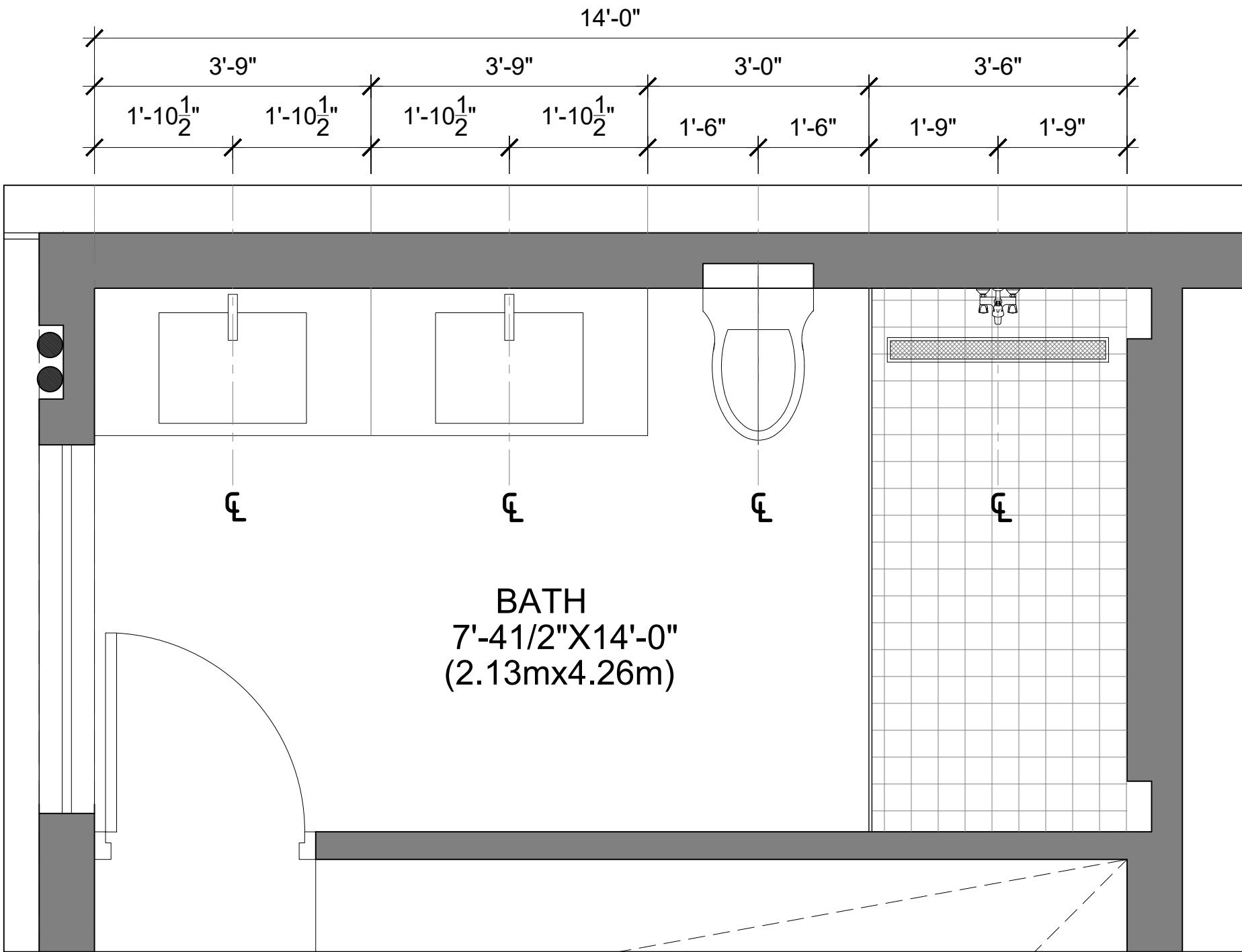
1 GROUND FLOOR BATH 1
