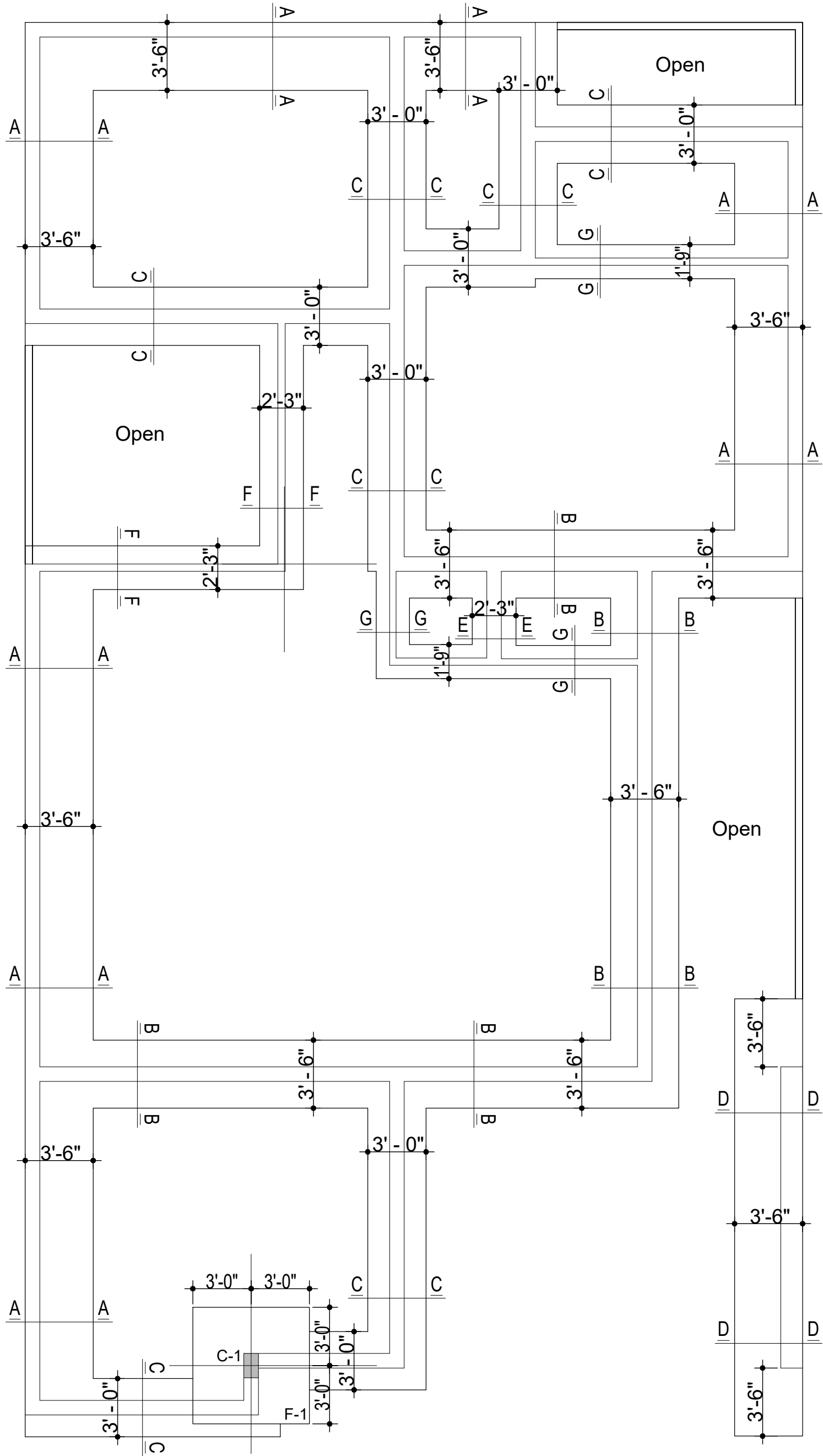
Foundation Plan
