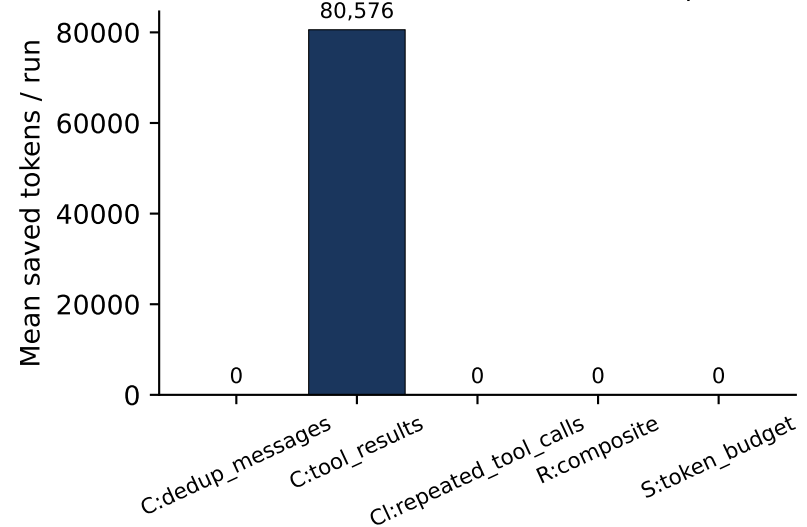
Token attribution (100 runs, balanced preset)
