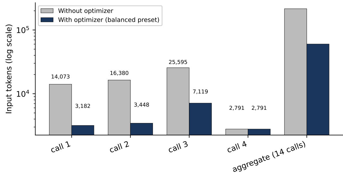
Per-call input tokens before vs. after ContextOptimizer (72.0% aggregate reduction)
