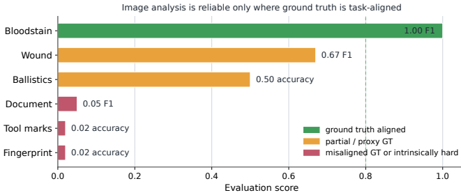
Fig. 7. Image analysis is reliable only where ground truth is task-aligned. Bloodstain (physics-grounded) succeeds; tasks with misaligned or proxy ground truth, or that are intrinsically hard from a single image, do not.
