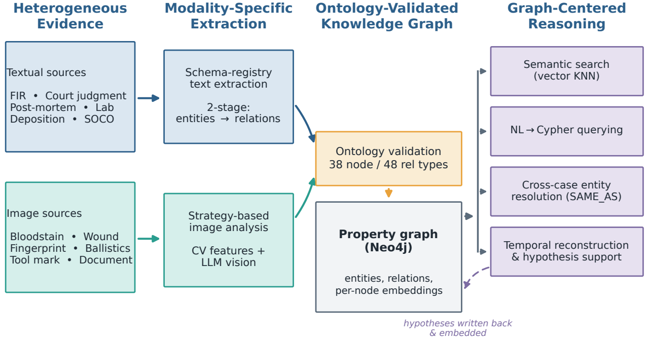
Fig. 1. End-to-end architecture. Textual and visual evidence are extracted by modality-specific components, type-checked against the forensic ontology, materialised in an embedded property graph, and consumed by semantic search, NL-to-Cypher querying, cross-case entity resolution, temporal reconstruction, and hypothesis support. Derived artefacts are written back and embedded.
