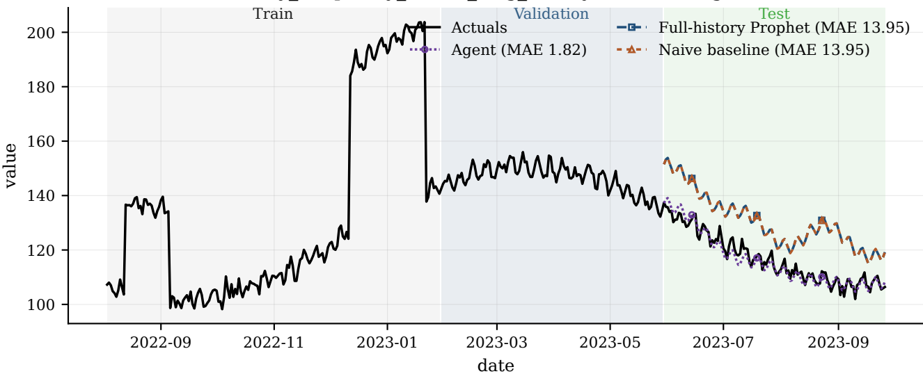
many_temporary_events_long_history — winner: agent
