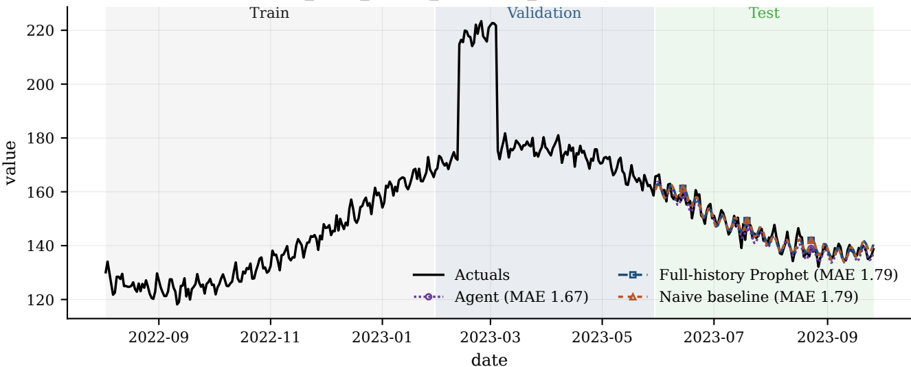
prophet_prior_tuning_recurring_event — winner: agent
