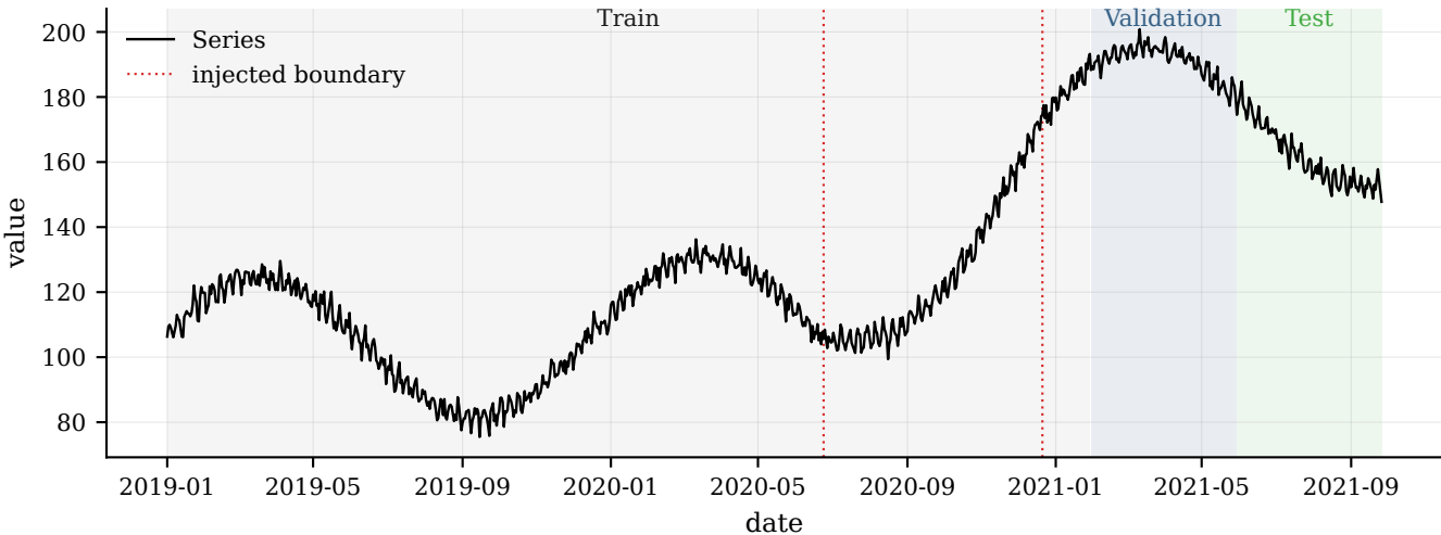
Gradual drift over a long transition with short post-drift seasonal history
