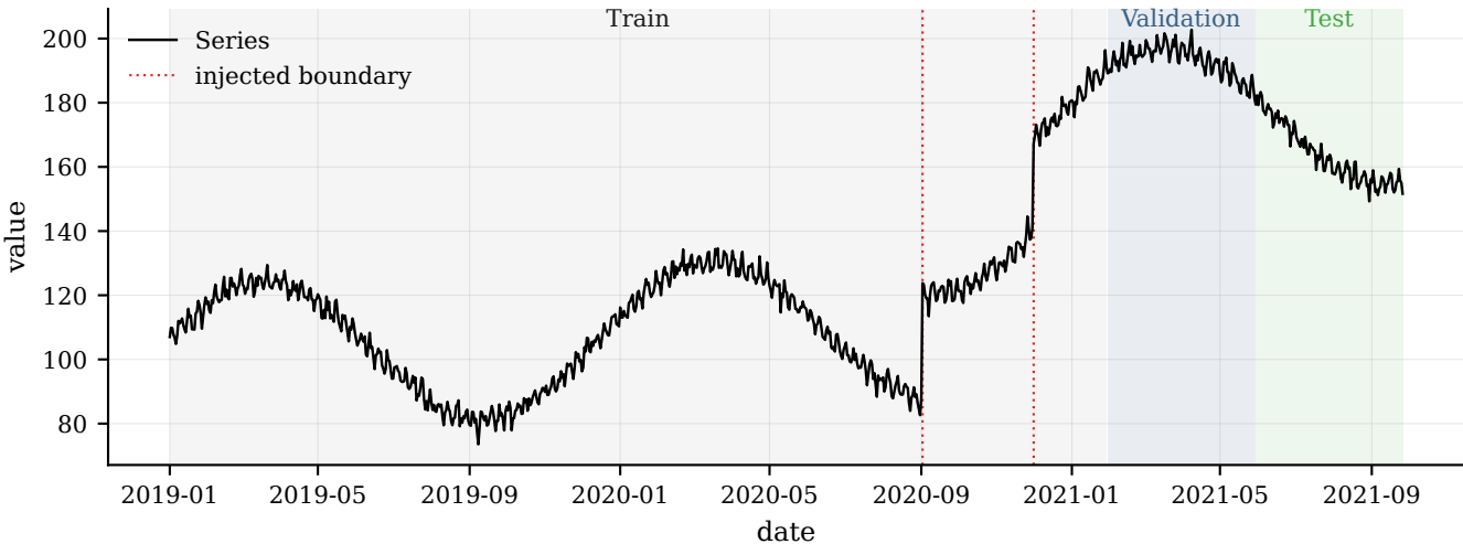
Multiple permanent level shifts with short post-change seasonal history
