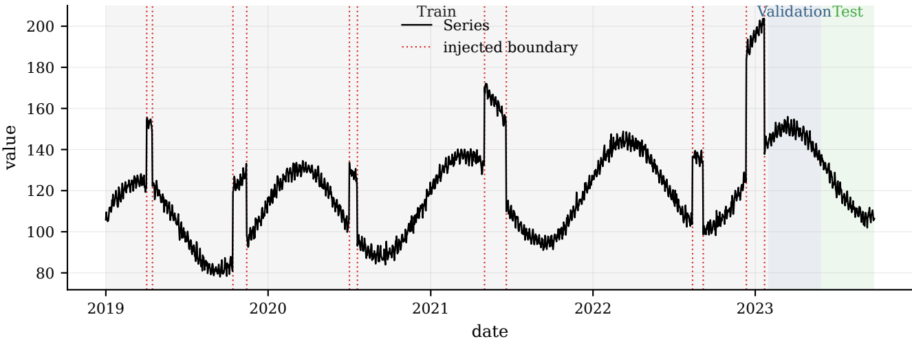
Six temporary events over longer history misread as changepoints
