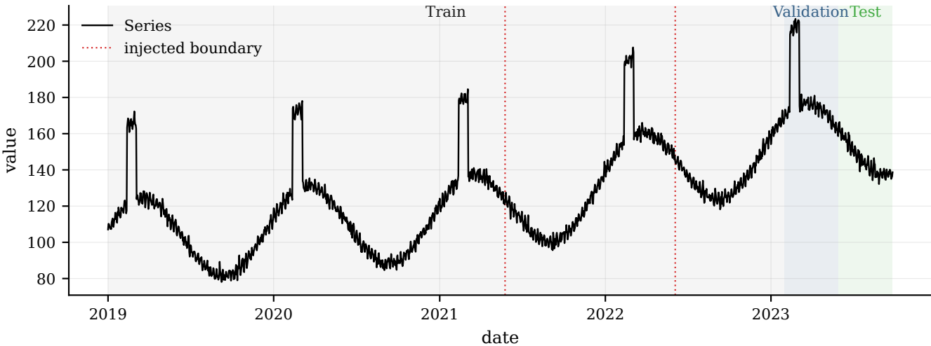
Recurring event plus trend kinks needs Prophet prior tuning
