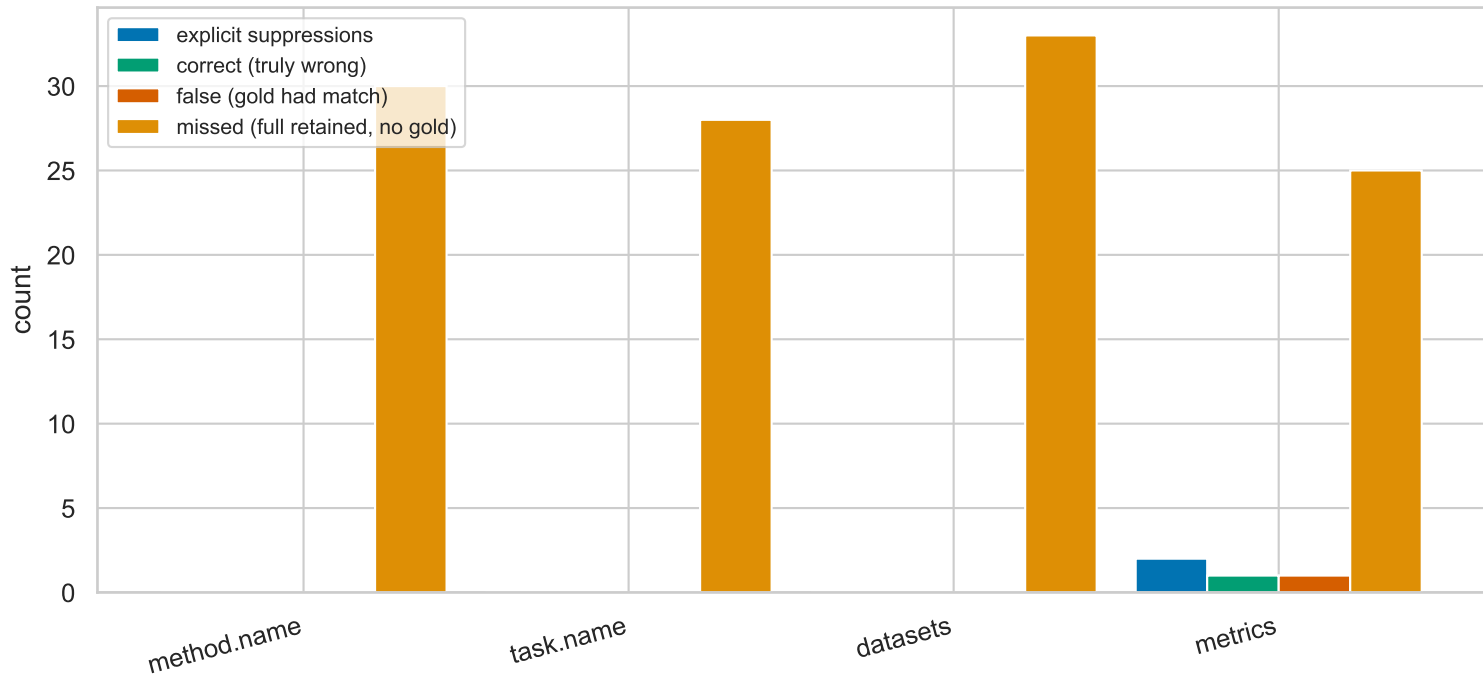
Critic suppression behaviour on SciREX dev (n=54)
