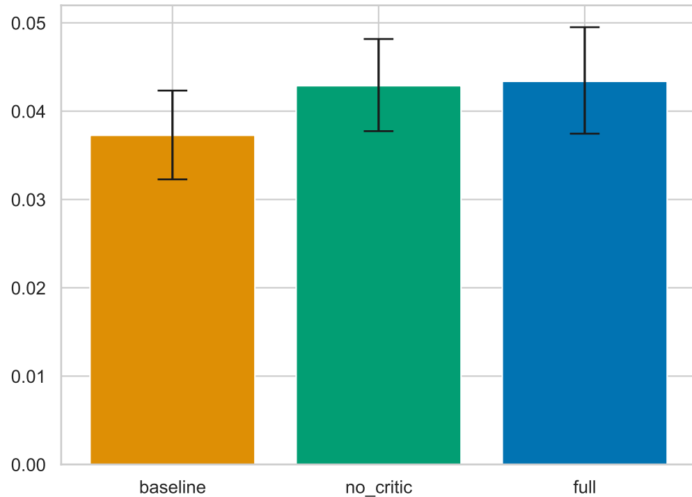
Resolved (string-match in source text)
