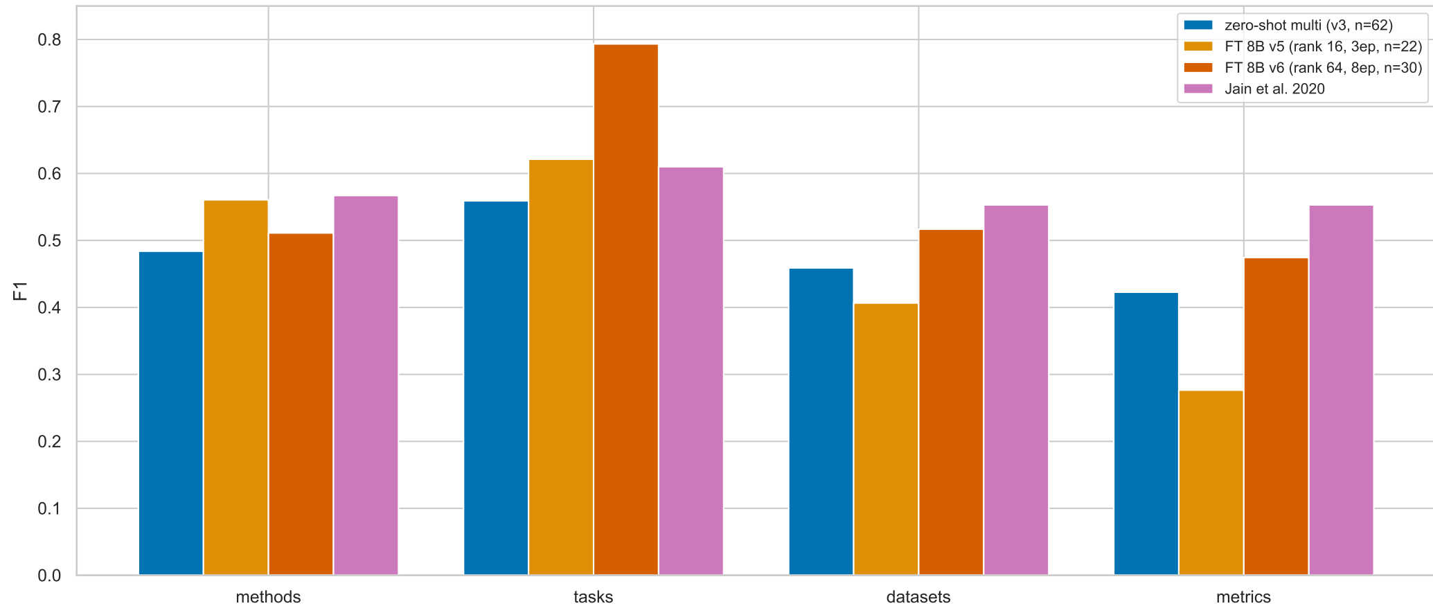
SciREX dev — multi-agent FT progression vs published prior
