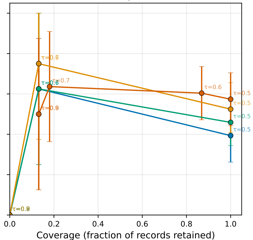
Confidence: temperature-scaled
