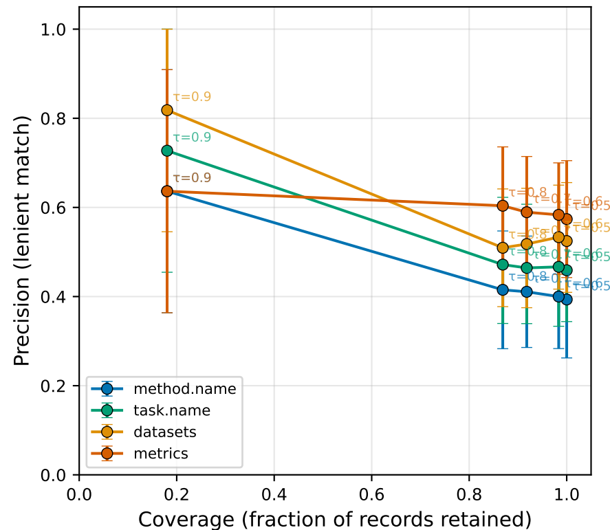
Confidence: uncalibrated
