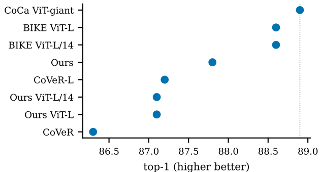
Kinetics-400
