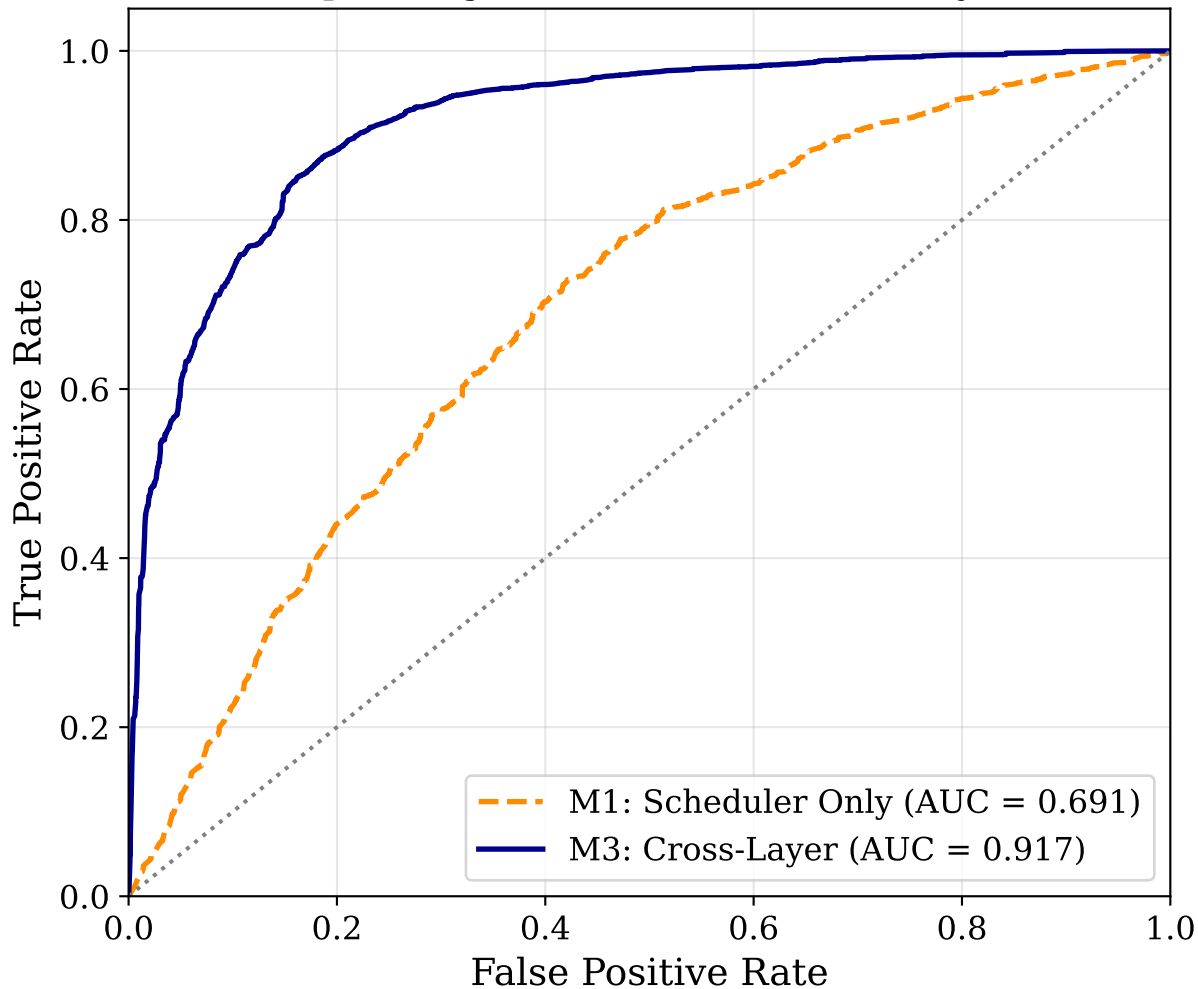
Receiver Operating Characteristic: Efficiency Prediction
