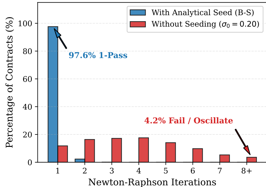
(a) Iteration Count Distribution
