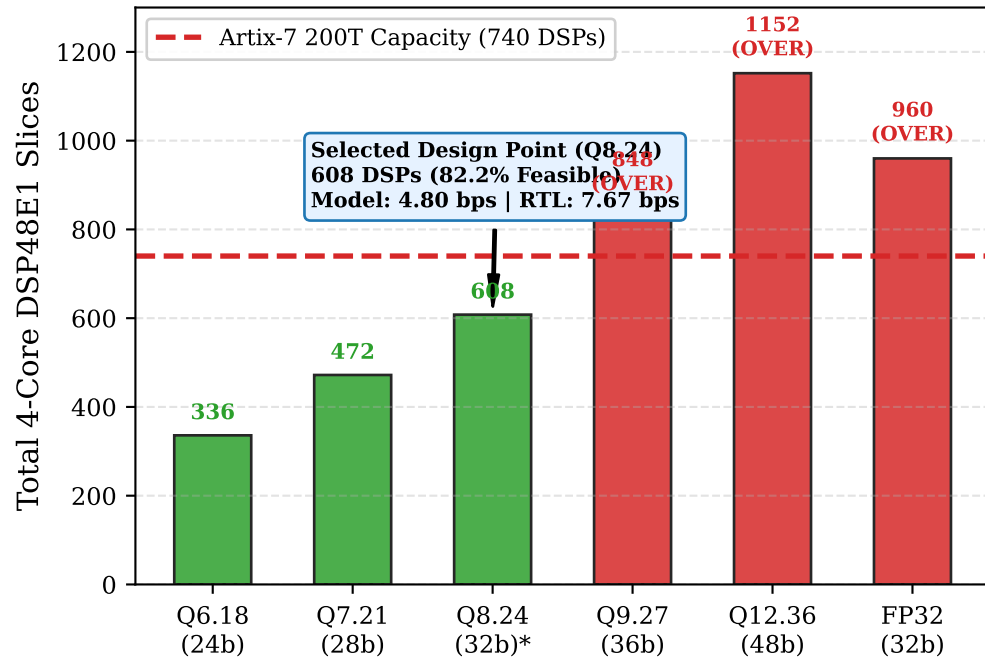
(b) Physical DSP Consumption vs. Device Capacity
