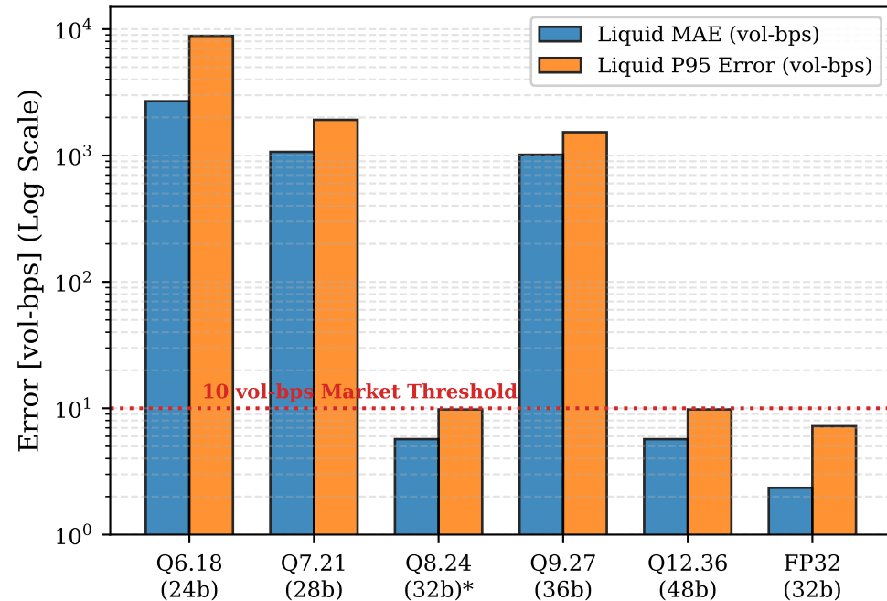
(a) Numerical Accuracy Across Wordlengths
