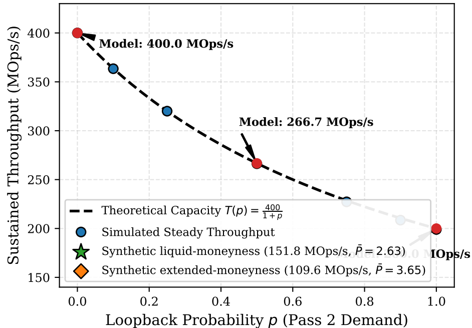
(a) Throughput vs. Loopback Probability ( || = 1, 4 Cores)
