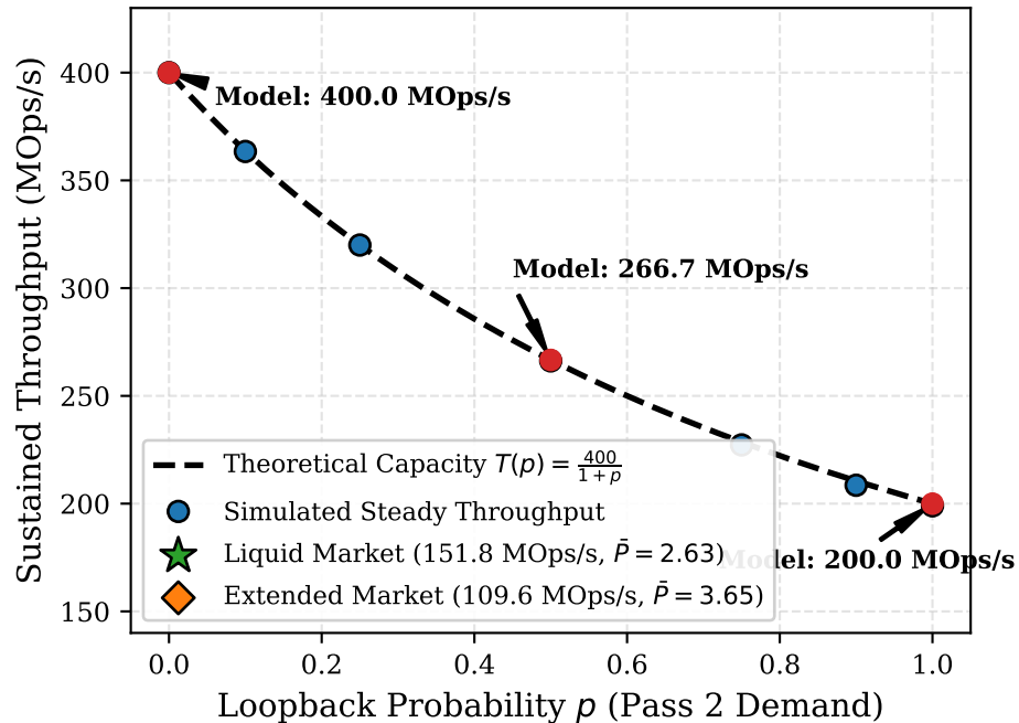
(a) Throughput vs. Loopback Probability ( || = 1, 4 Cores)
