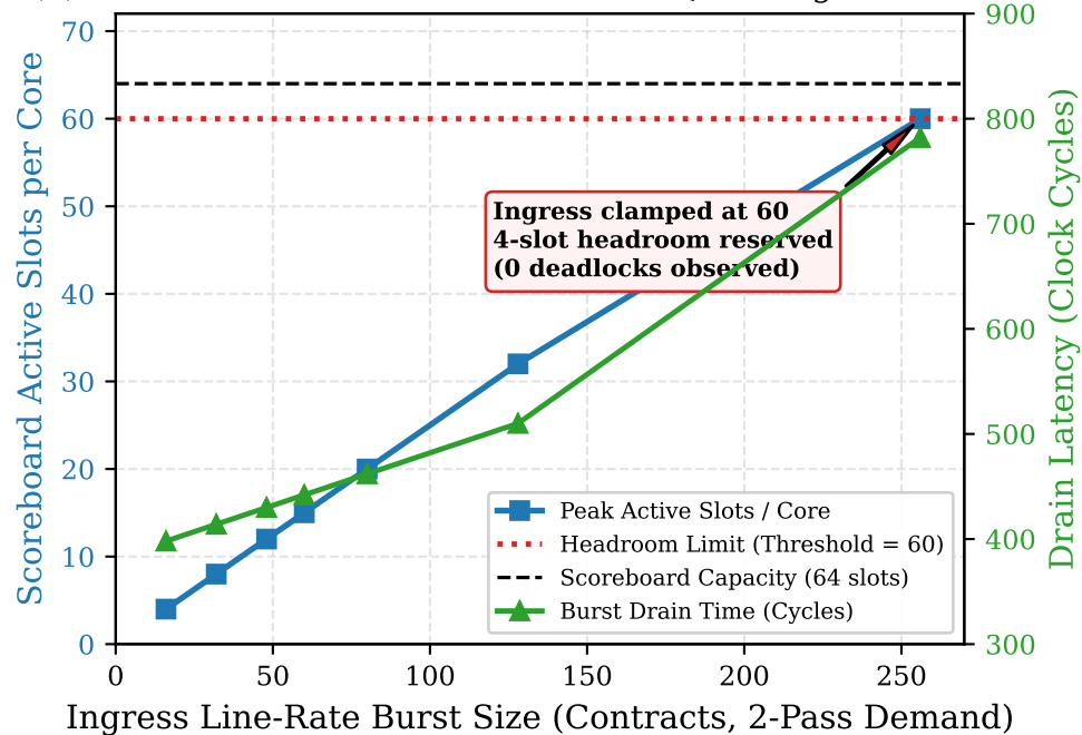
(b) Scoreboard Headroom & Bounded Queueing Under Burst
