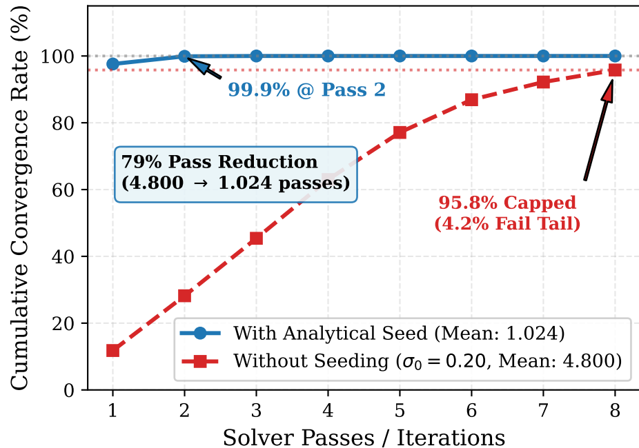
(b) Cumulative Convergence CDF
