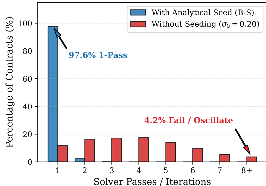
(a) Pass Count Distribution
