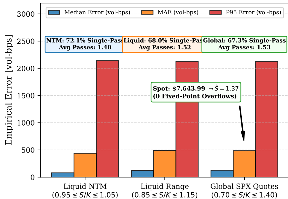
(b) CBOE European SPX Scale-Invariance ( N = 1,382 )
