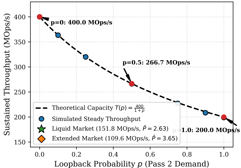
(a) Throughput vs. Loopback Probability ( l = 1, 4 Cores)
