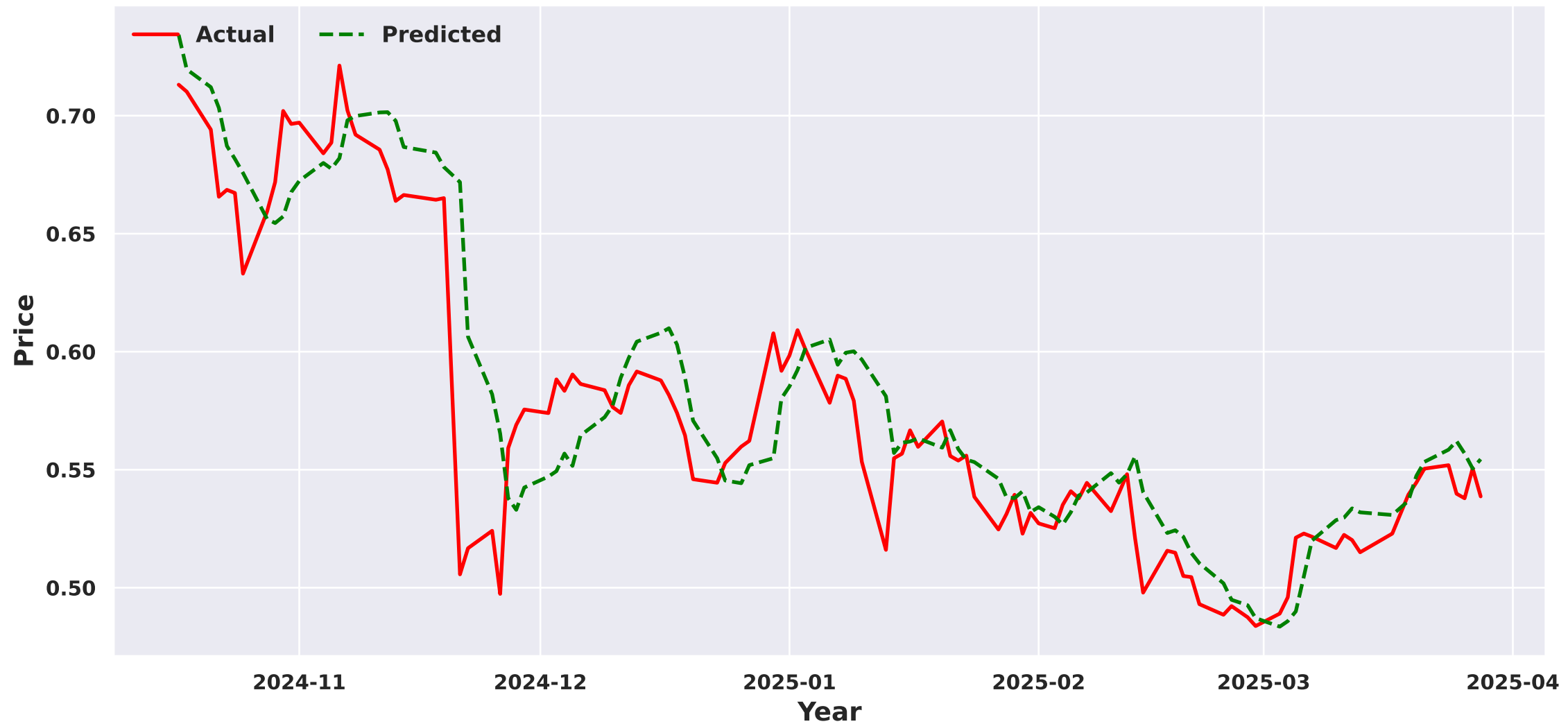
Adani Enterprises - Bi-LSTM Prediction on Test set
