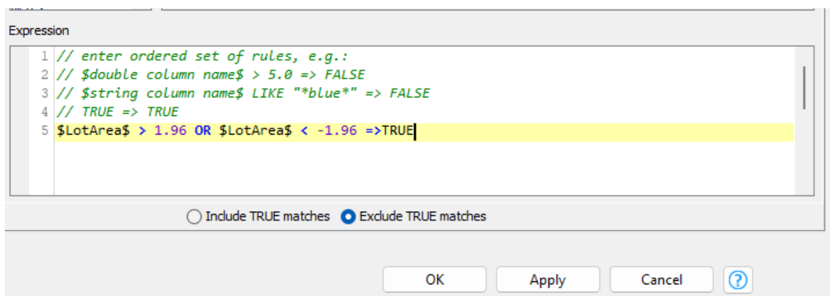
Figure 15: Exclude all rows that match the condition
