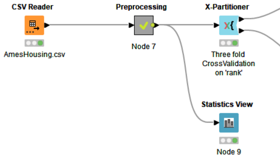
Figure 6: Try with three-fold, five-fold and 10-fold classification.
