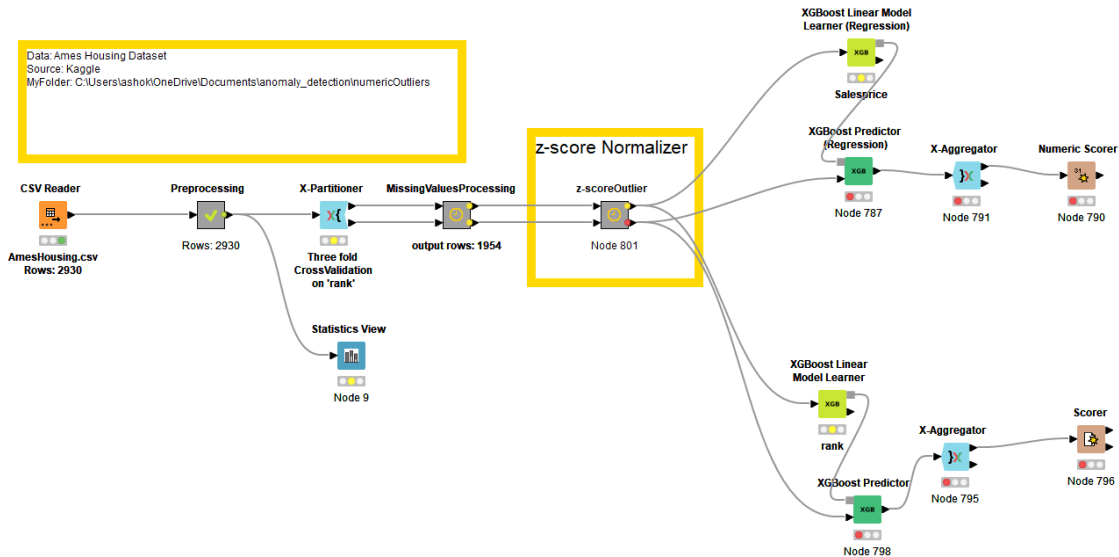
Figure 16: We get better results for Saleprice prediction
