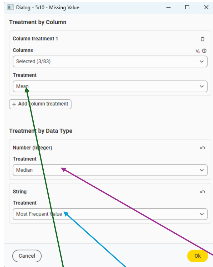
Figure 11: For three columns, we select Mean as the filler. For the remaining number type, we select Median as the filler and for all String types we select Mode as the filler.
