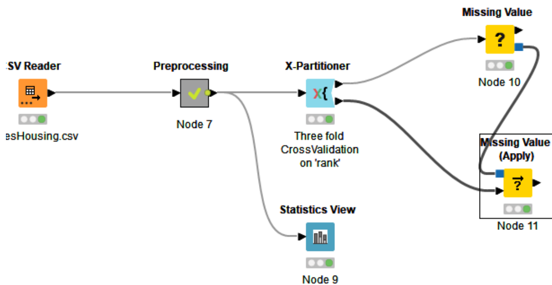
Figure 12: We will shortly put both the Missing value nodes in a Metanode.
