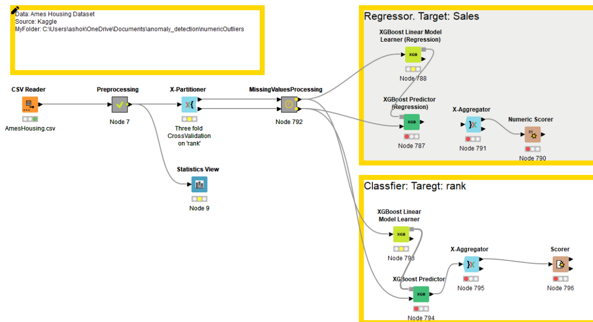
Figure 13: Complete Configuration for two kinds of cases: Regression and Classification
