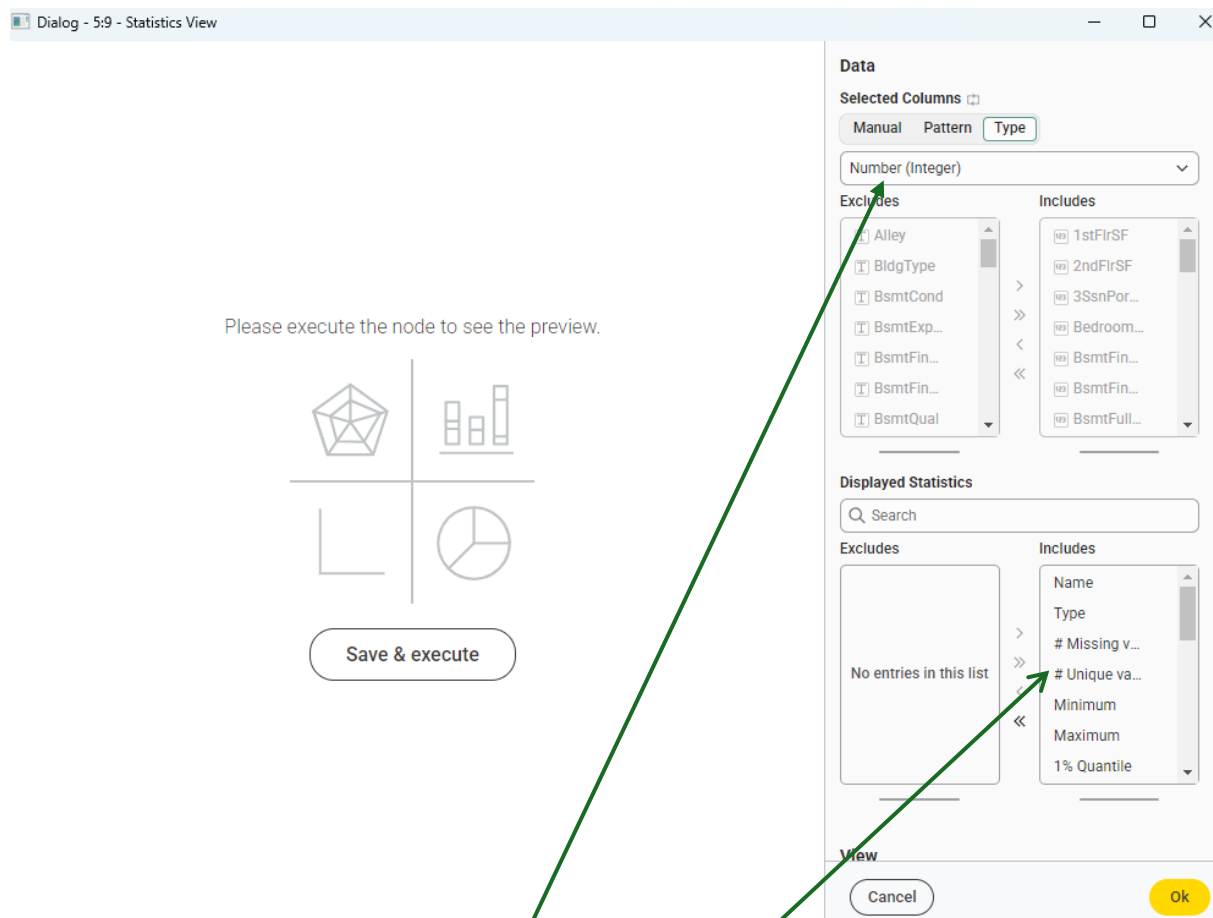
Figure 7: Configure first for columns with Type->Number and we select all statistics. Click OK.
