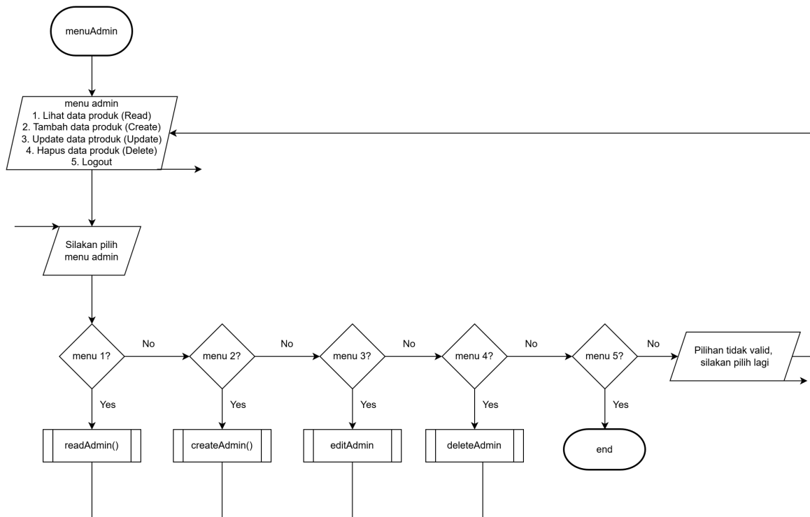
1.4 flowchart menu admin
