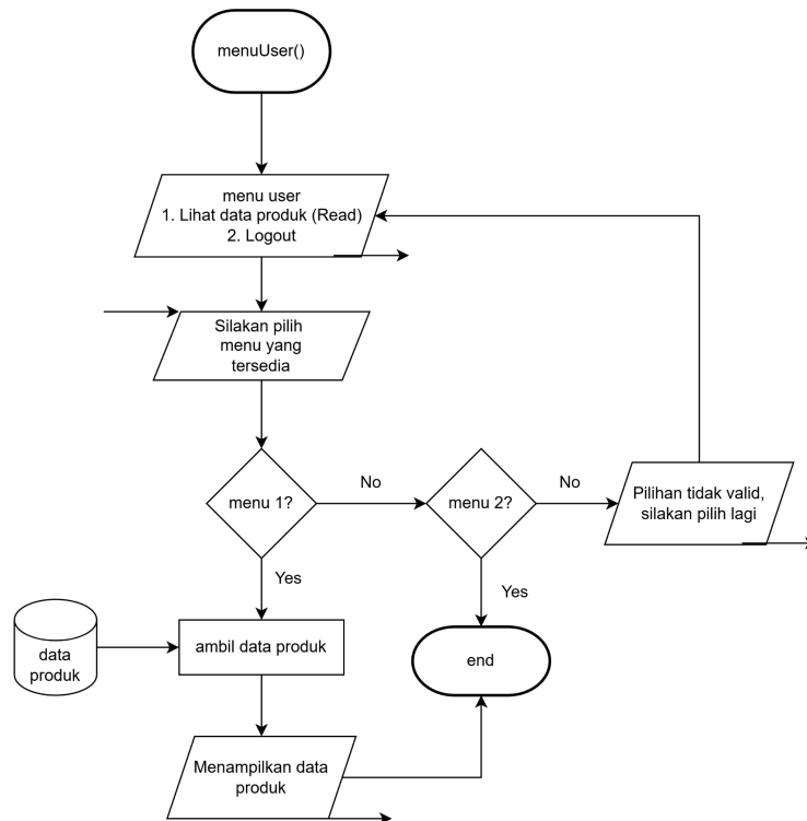
1.7 flowchart menu user
