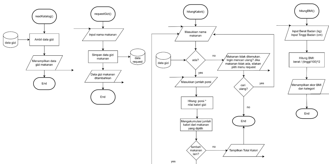
Flowchart 2.12 Menu read, request, kalkulator kalori, dan kalkulator BMI
