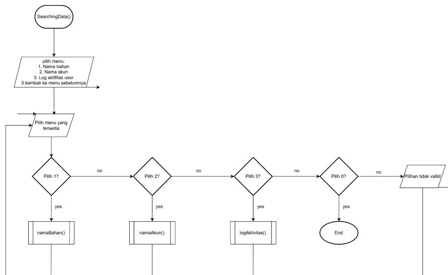
Flowchart 2.9 Menu searching admin
