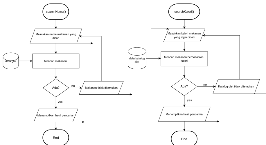
Flowchart 2.18 Menu searching user
