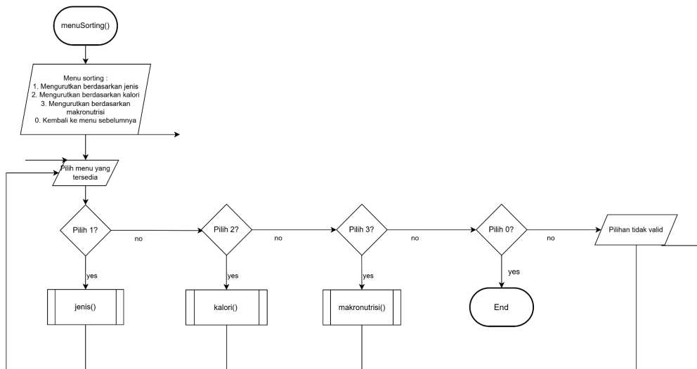
Flowchart 2.13 Menu sorting user
