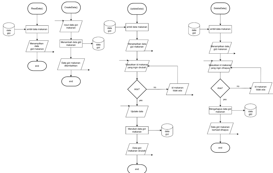
Flowchart 2.5 Menu read, create, update, dan delete
