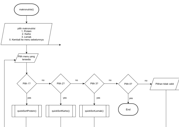
Flowchart 2.15 Menu sorting user berdasarkan makronutrisi
