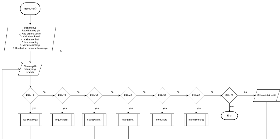
Flowchart 2.11 Menu user
