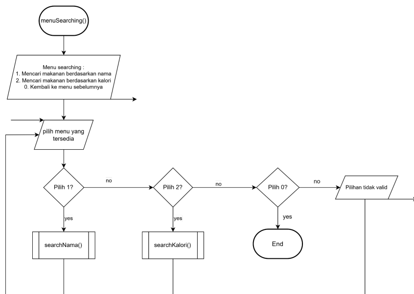
Flowchart 2.17 Menu searching
