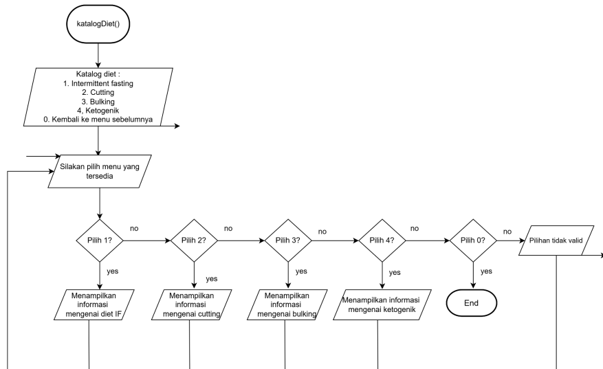
Flowchart 2.3 Menu katalog diet
