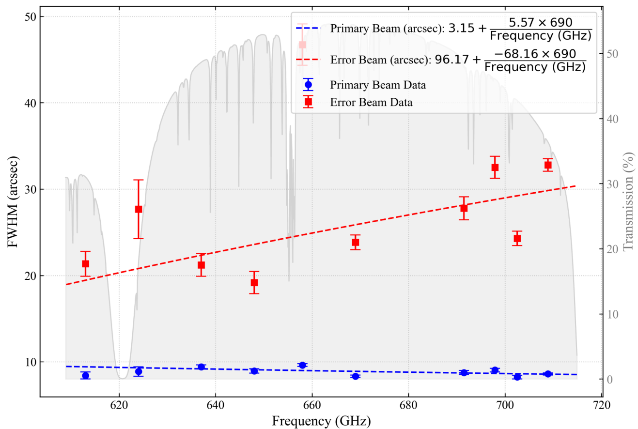
Figure 2. Beam Size measurement results. The blue and red data points represent the measurement of the primary and secondary beam. Their respective linear fits are presented as the dashed lines and their values in the figure inset. The grey right axis and plot in the background show the atmospheric transmission at Mauna Kea, showing the notable water vapor absorption lines.
