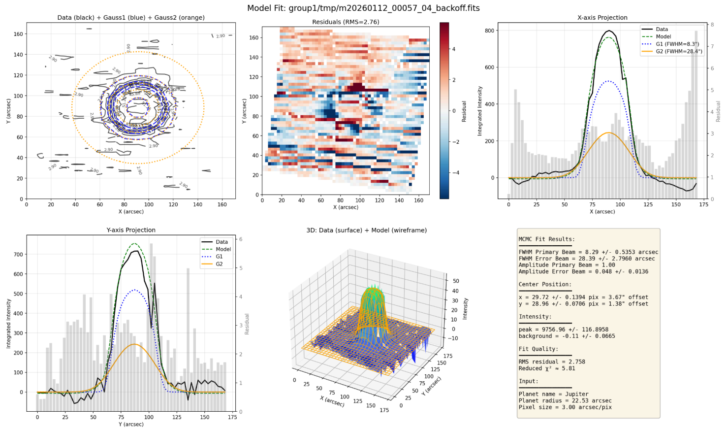
Figure 1. Example of the MCMC results for a single frequency measurement,. The model is shown in green and the data in black in the upper left, upper right and lower left panel. The top middle panel shows the residuals, calculated from subtracting the model to the data. The lower middle panel shows the 3D representation of the data and model. The lower right panel shows the numerical values of the results.
