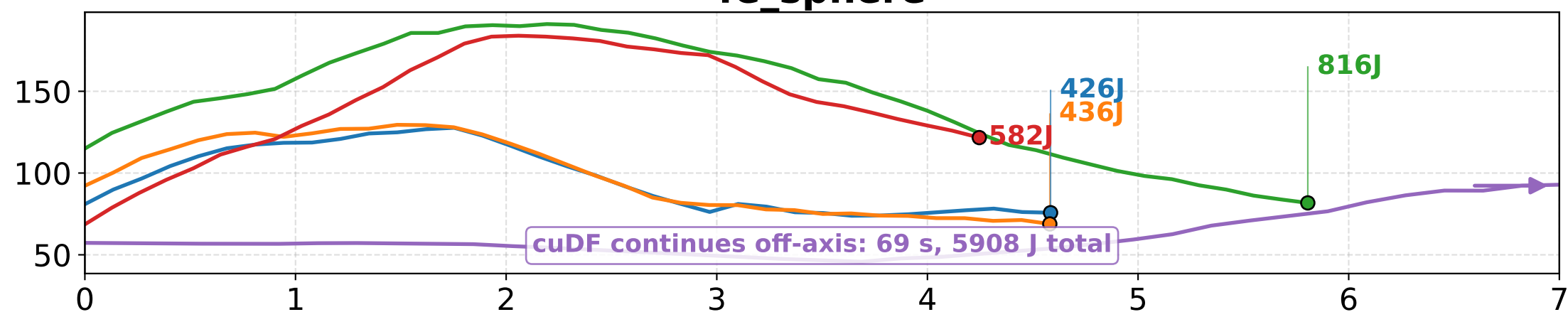
ca_hepth
