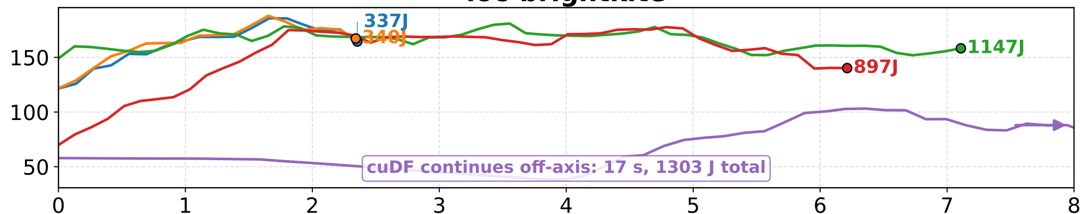
fe_sphere
