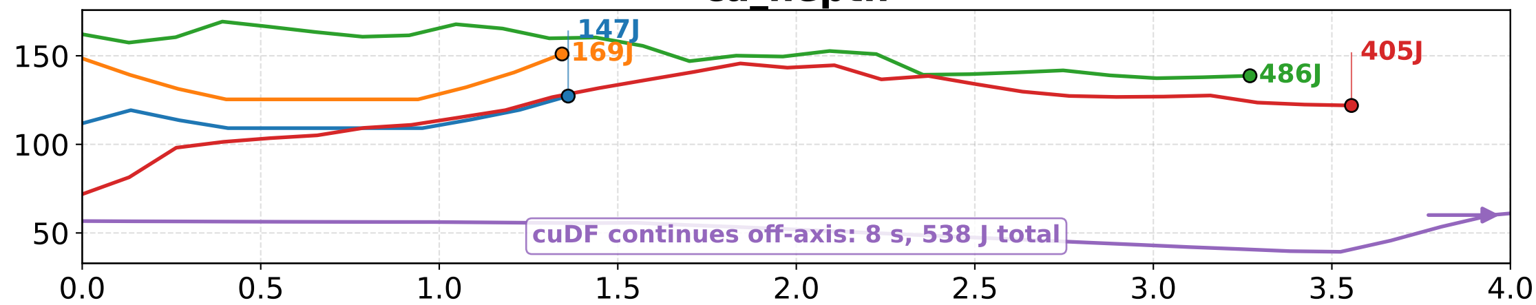
ca_hepth
