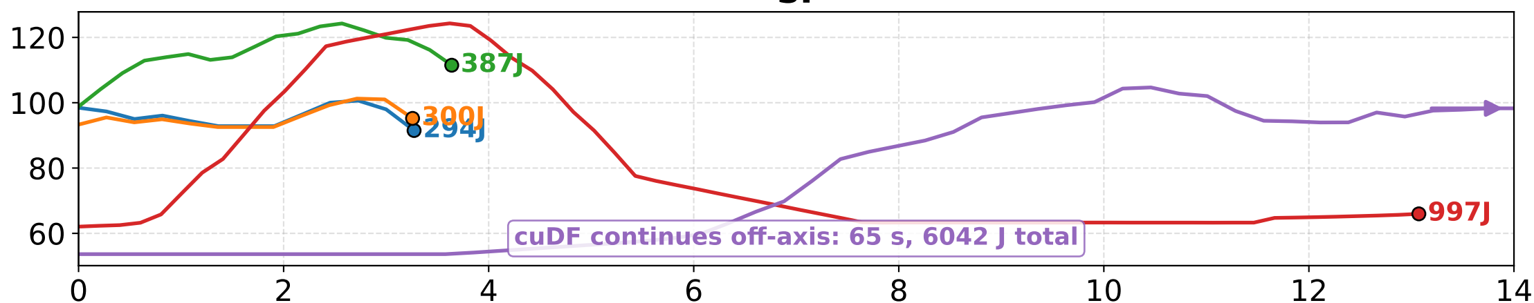
usroads
