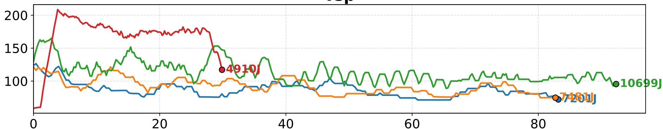
sf
