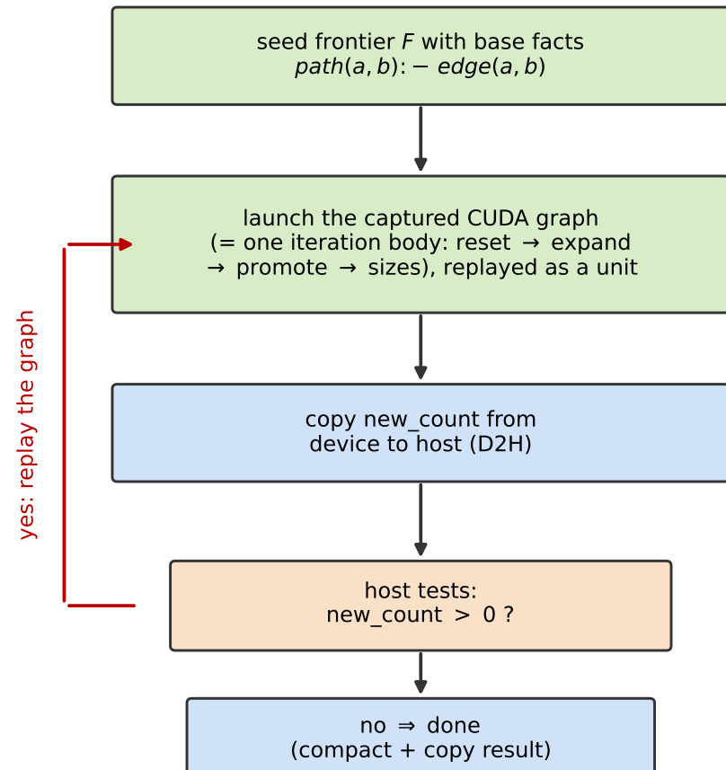
(b) replayed CUDA graph [fused+graph]
