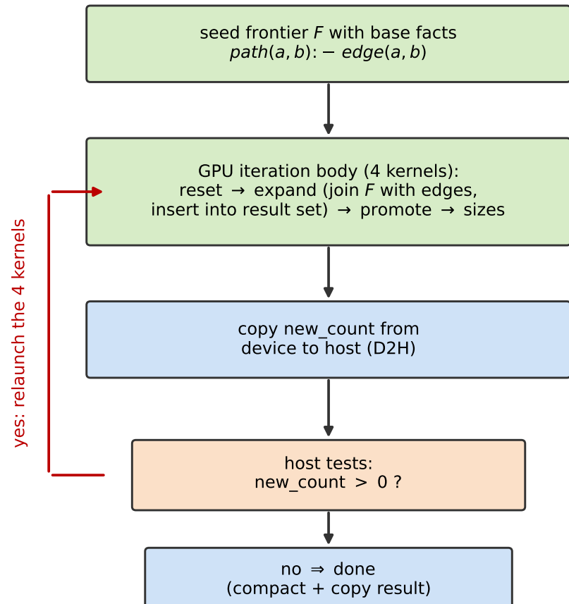
(a) host loop [MNMGDatalog, fused]
