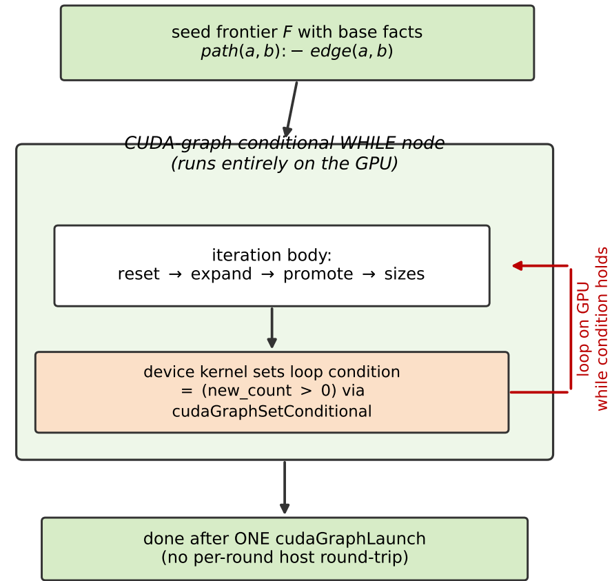
(c) conditional WHILE node [fused+cond]
