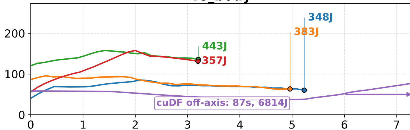
Transitive Closure (TC)
