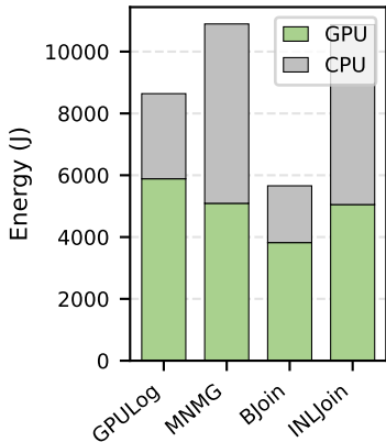
TC (usroads)
