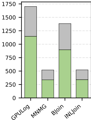
SG (loc-brightkite)
