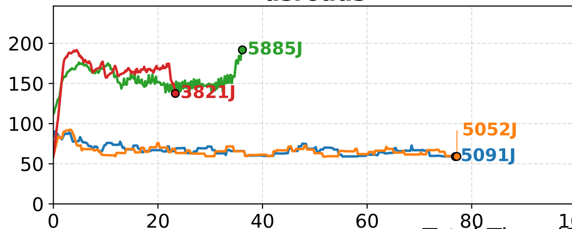
usroads
