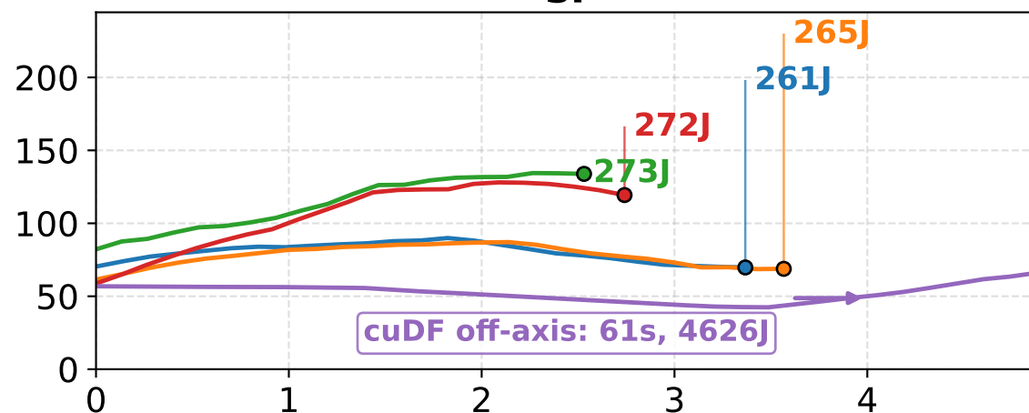
sf
