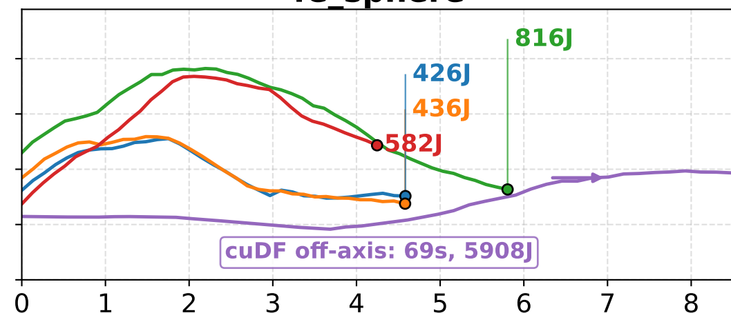
fe_sphere
