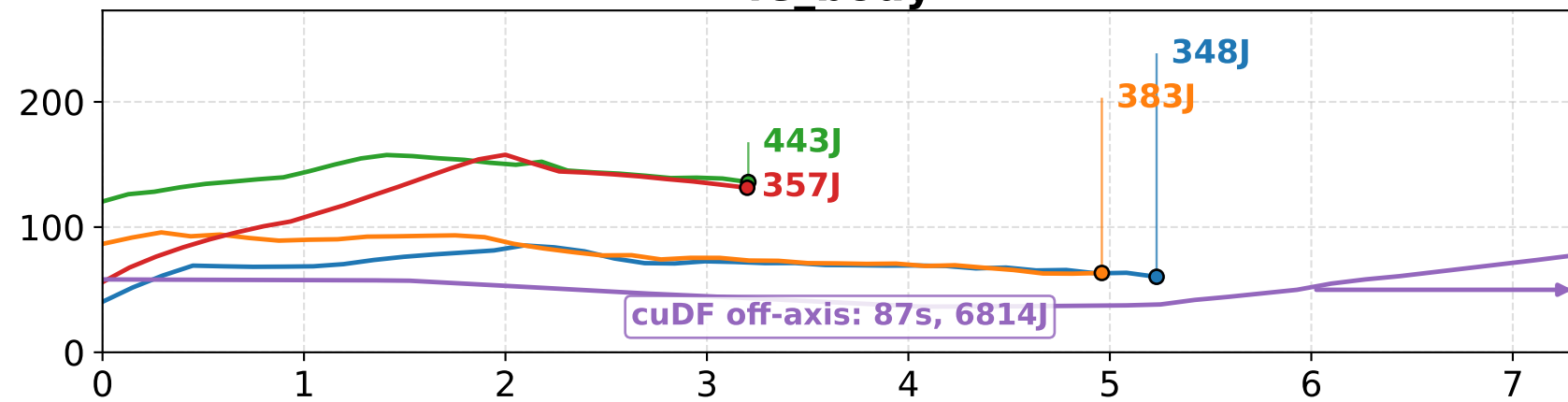
Transitive Closure (TC) fe_body
