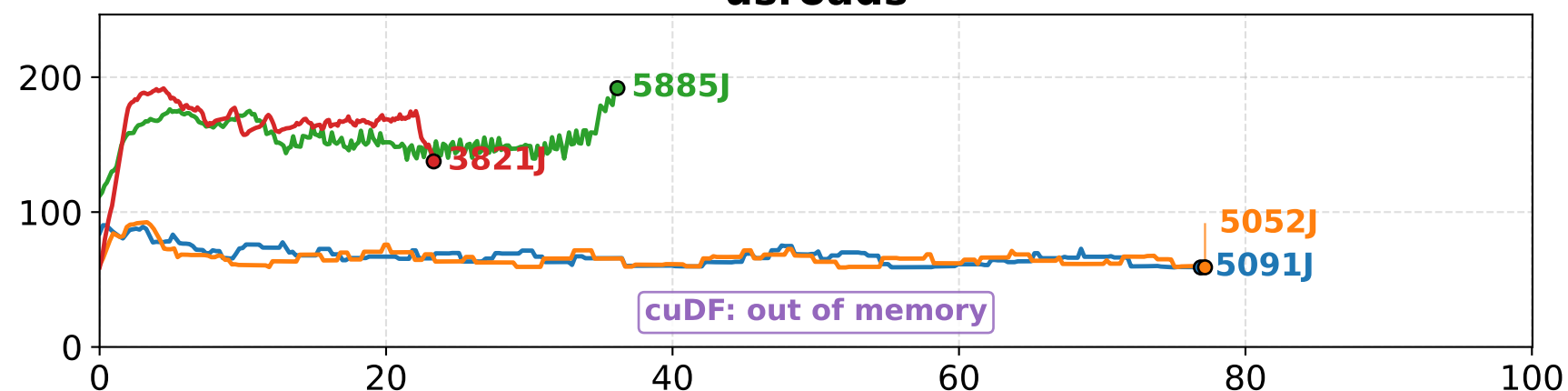
usroads
