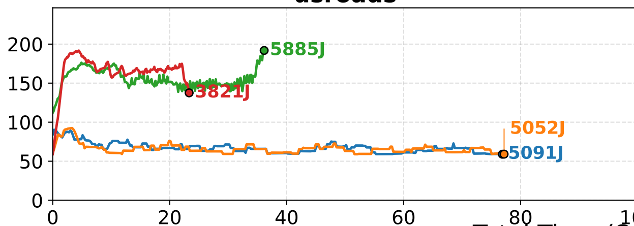
usroads
