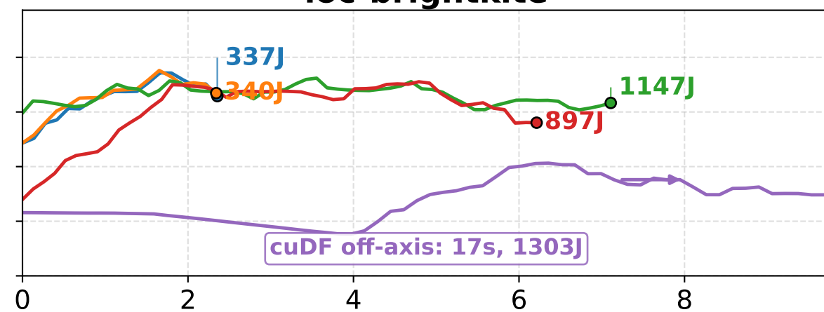
loc-brightkite
