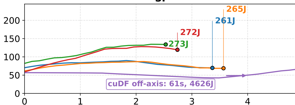
sf
