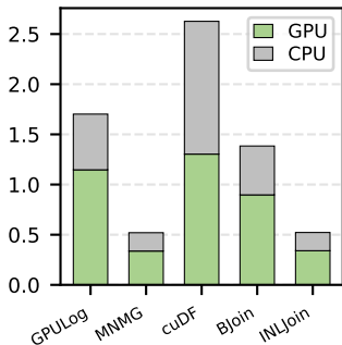
SG (loc-brightkite)
