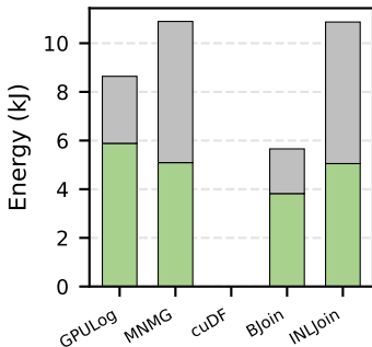
TC (usroads)
