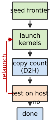
(a) host loop
