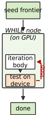
(c) cond. node
