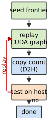
(b) CUDA graph
