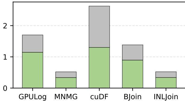
SG (loc-brightkite)
